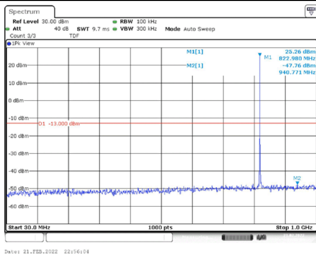
Band26-1.4MHz-16QAM-26783-1RB#0-Range1:30~1000MHz
