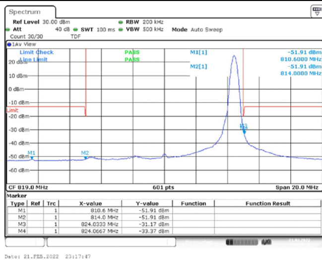
Band26-10MHz-16QAM-26740-1RB#49
