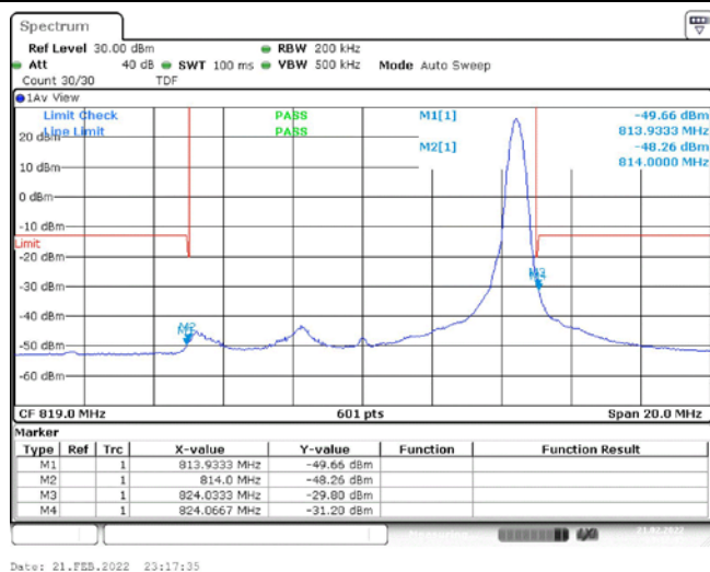
Band26-10MHz-QPSK-26740-1RB#49
