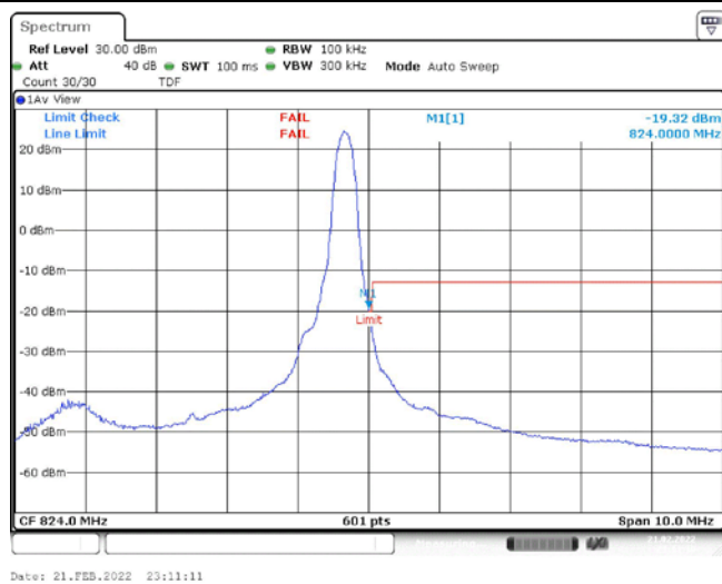
Band26-5MHz-QPSK-26765-1RB#24
