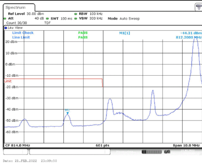
Band26-5MHz-QPSK-26715-1RB#24
