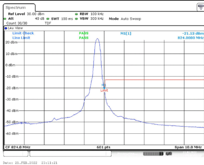
Band26-5MHz-16QAM-26765-1RB#24
