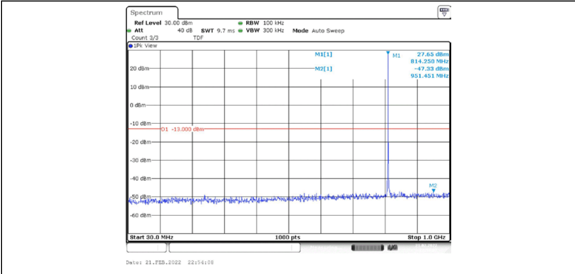
Band26-1.4MHz-QPSK-26697-1RB#0-Range1:30~1000MHz
