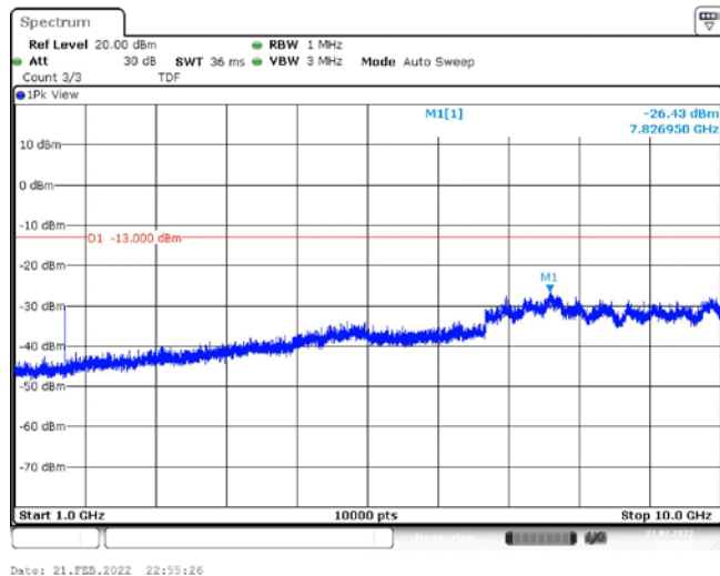
Band26-1.4MHz-16QAM-26740-1RB#0-Range2:1000~10000MHz
