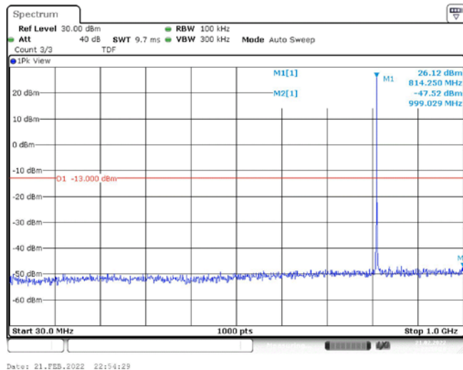
Band26-1.4MHz-16QAM-26697-1RB#0-Range1:30~1000MHz
