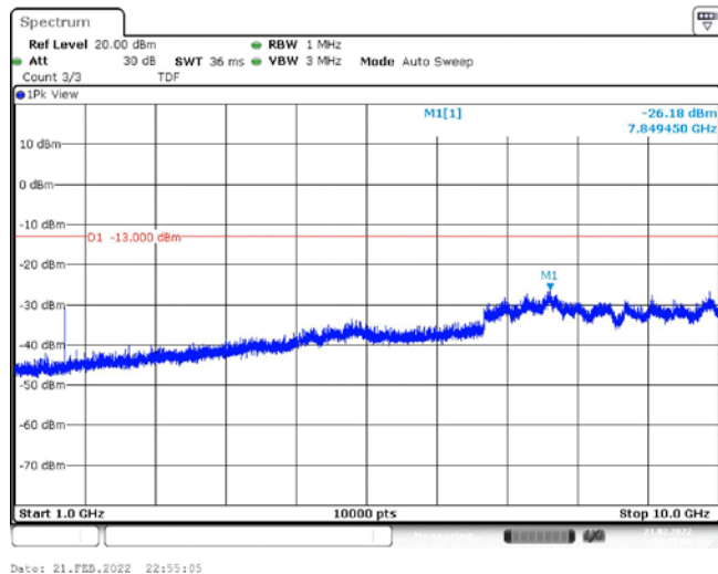
Band26-1.4MHz-QPSK-26740-1RB#0-Range2:1000~10000MHz
