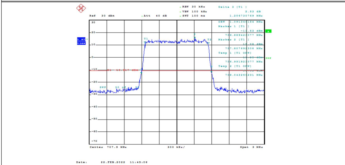
Band12-1.4MHz-QPSK-23095-6RB#0-1.091
