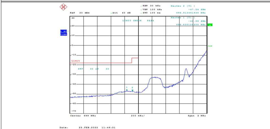
Band12-1.4MHz-QPSK-23017-1RB#5
