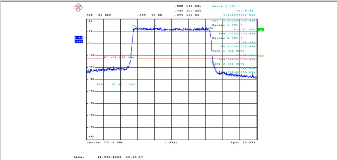
Band12-5MHz-QPSK-23035-25RB#0-4.512
