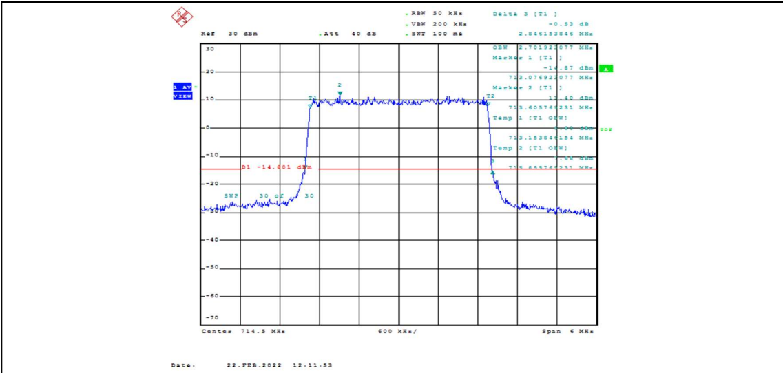
Band12-3MHz-16QAM-23165-15RB#0-2.702
