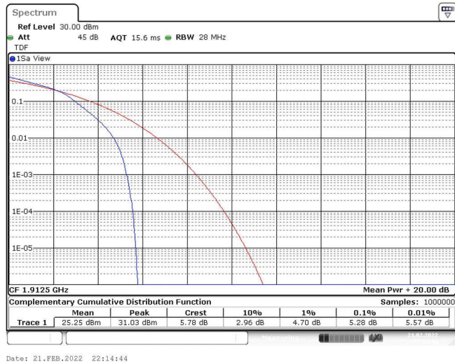
Band25-5MHz-16QAM-26665-25RB#0
