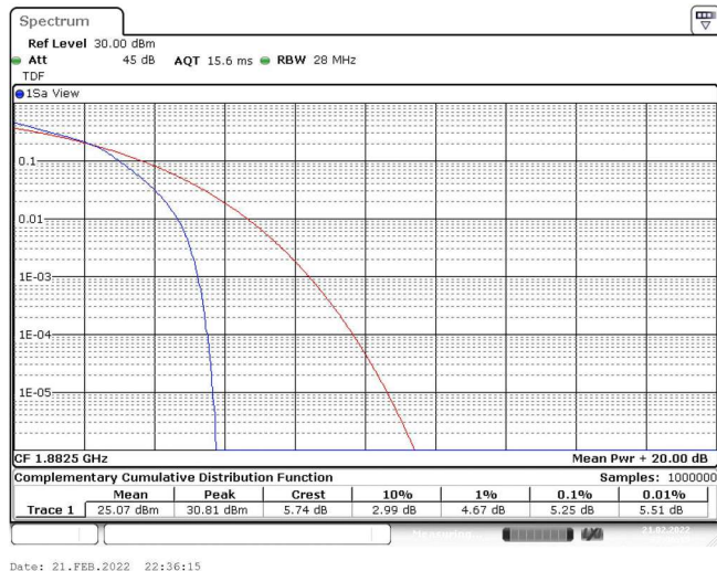
Band25-15MHz-16QAM-26365-75RB#0
