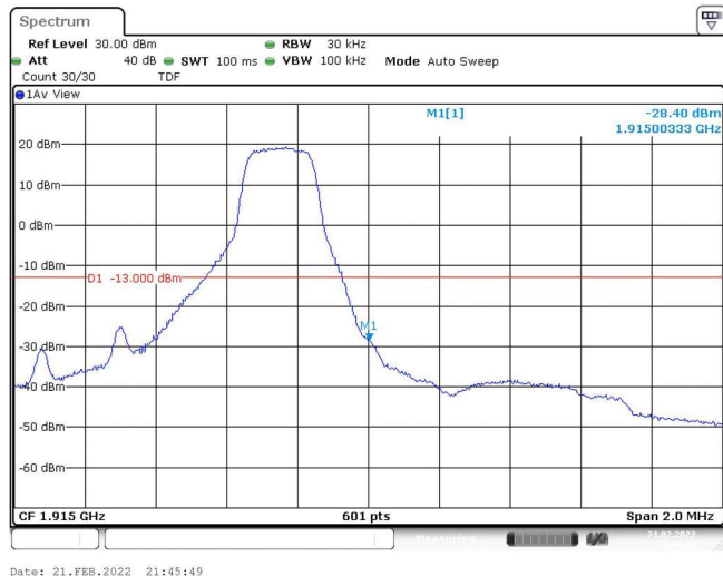
Band25-1.4MHz-QPSK-26683-1RB#5
