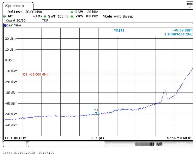
Band25-1.4MHz-16QAM-26047-1RB#5
