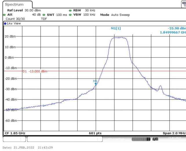
Band25-1.4MHz-QPSK-26047-1RB#0
