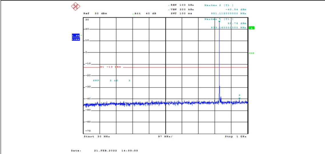
Band26-10MHz-QPSK-26915-1RB#0-Range1:30~1000MHz
