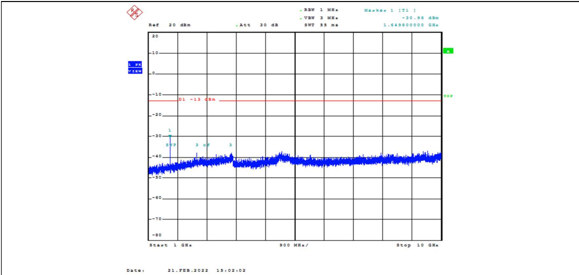
Band26-15MHz-QPSK-26865-1RB#0-Range2:1000~10000MHz
