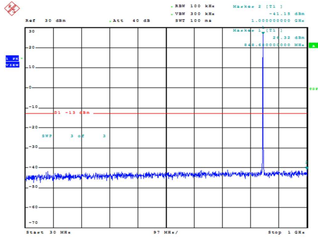
Band26-1.4MHz-QPSK-27033-1RB#0-Range1:30~1000MHz
