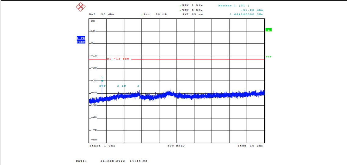
Band26-10MHz-QPSK-26915-1RB#0-Range2:1000~10000MHz
