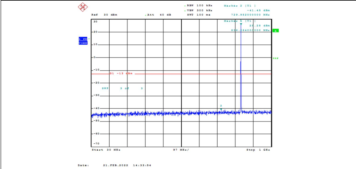
Band26-1.4MHz-16QAM-26915-1RB#0-Range1:30~1000MHz
