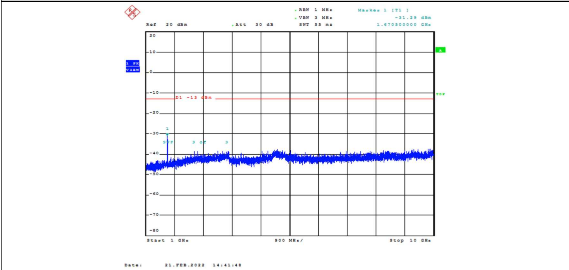
Band26-3MHz-QPSK-26915-1RB#0-Range2:1000~10000MHz
