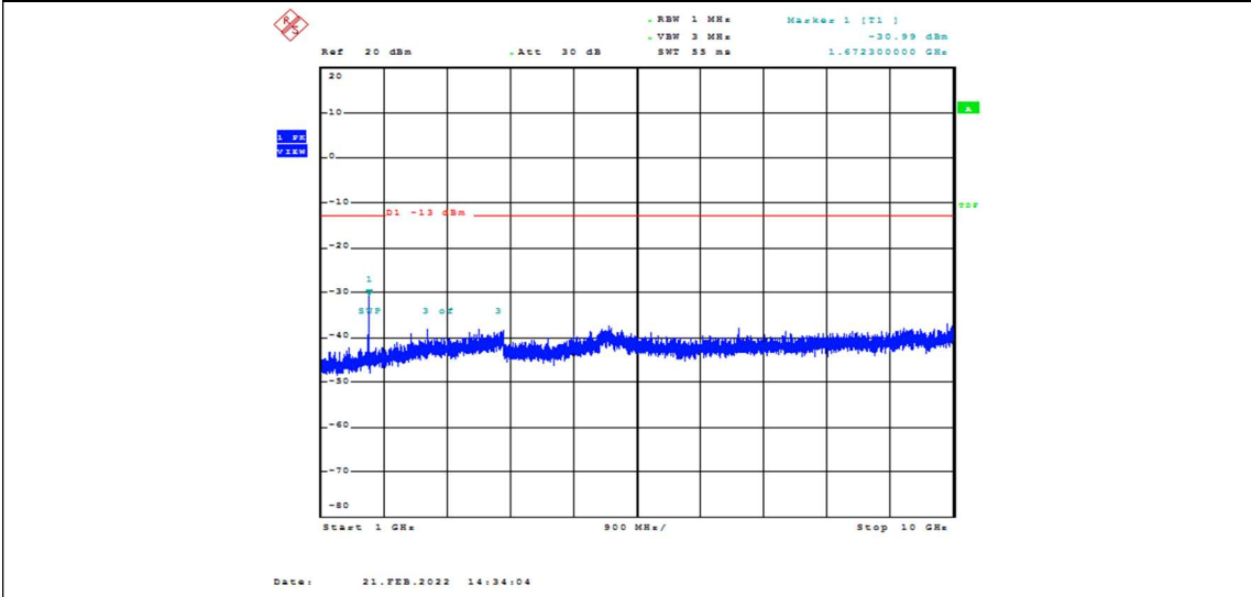
Band26-1.4MHz-16QAM-26915-1RB#0-Range2:1000~10000MHz
