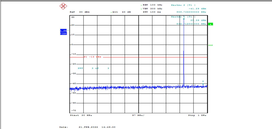
Band26-5MHz-16QAM-26915-1RB#0-Range1:30~1000MHz
