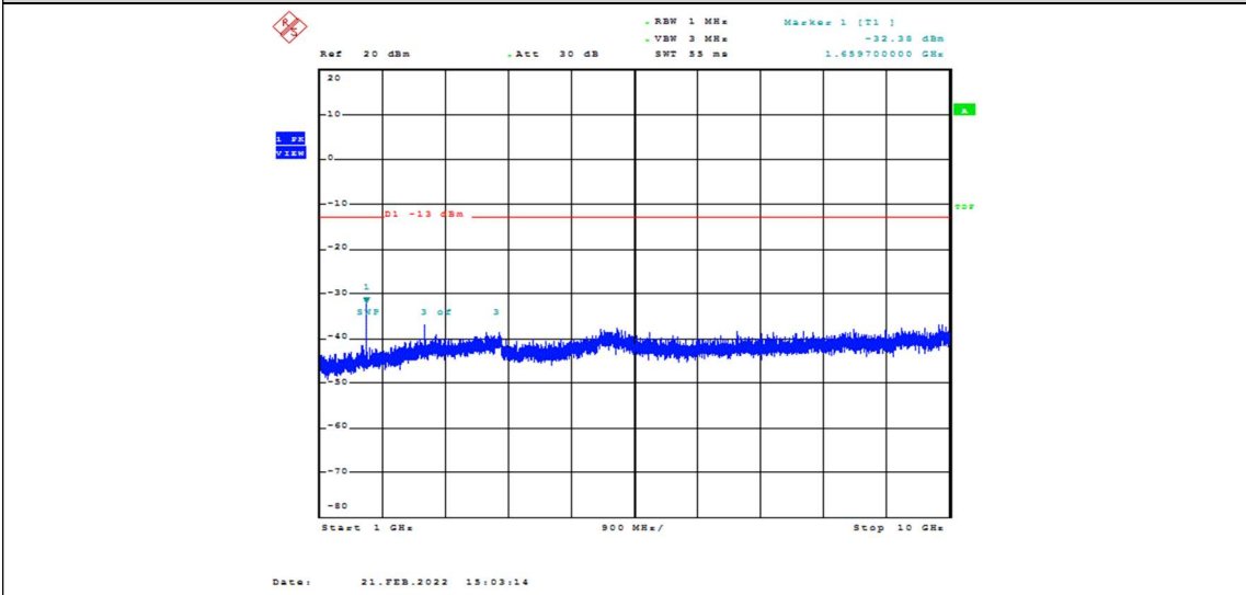
Band26-15MHz-16QAM-26915-1RB#0-Range2: 1000~10000MHz
