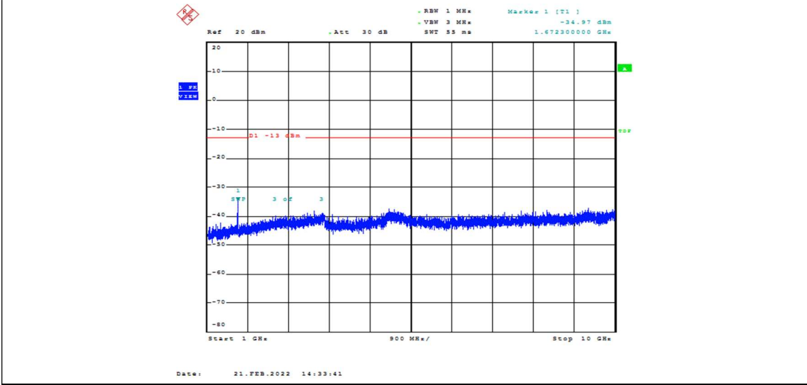
Band26-1.4MHz-QPSK-26915-1RB#0-Range2:1000~10000MHz
