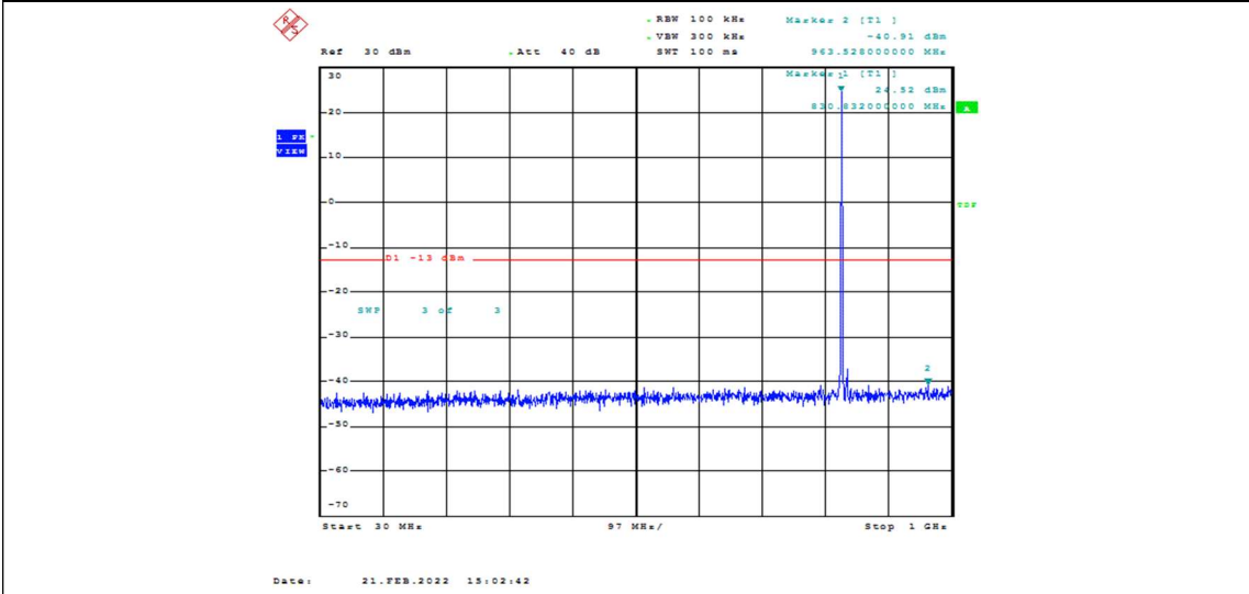
Band26-15MHz-QPSK-26915-1RB#0-Range1:30~1000MHz
