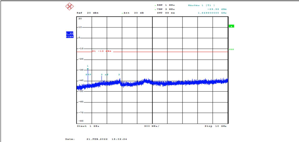
Band26-15MHz-16QAM-26865-1RB#0-Range2: 1000~10000MHz
