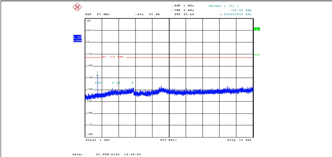
Band26-5MHz-16QAM-26815-1RB#0-Range2:1000~10000MHz
