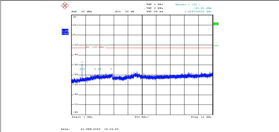
Band26-15MHz-QPSK-26915-1RB#0-Range2:1000~10000MHz
