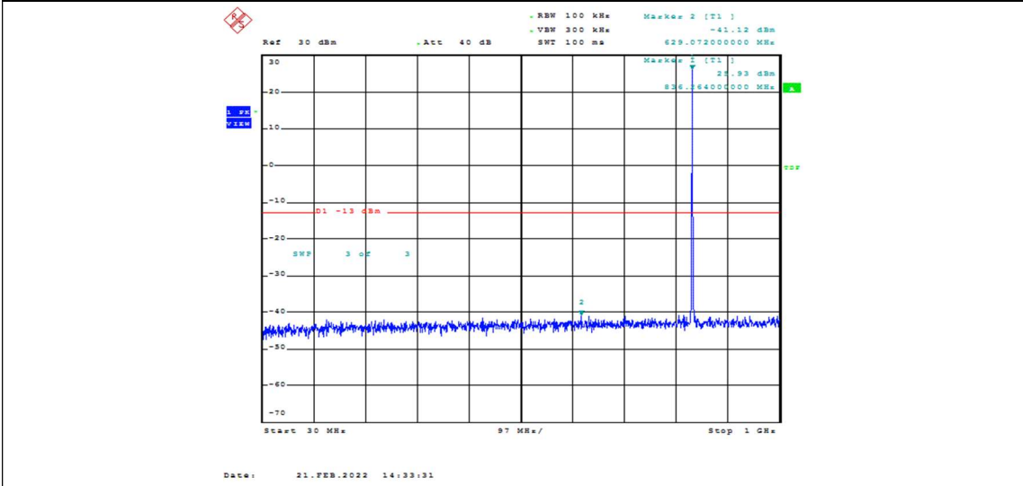
Band26-1.4MHz-QPSK-26915-1RB#0-Range1:30~1000MHz
