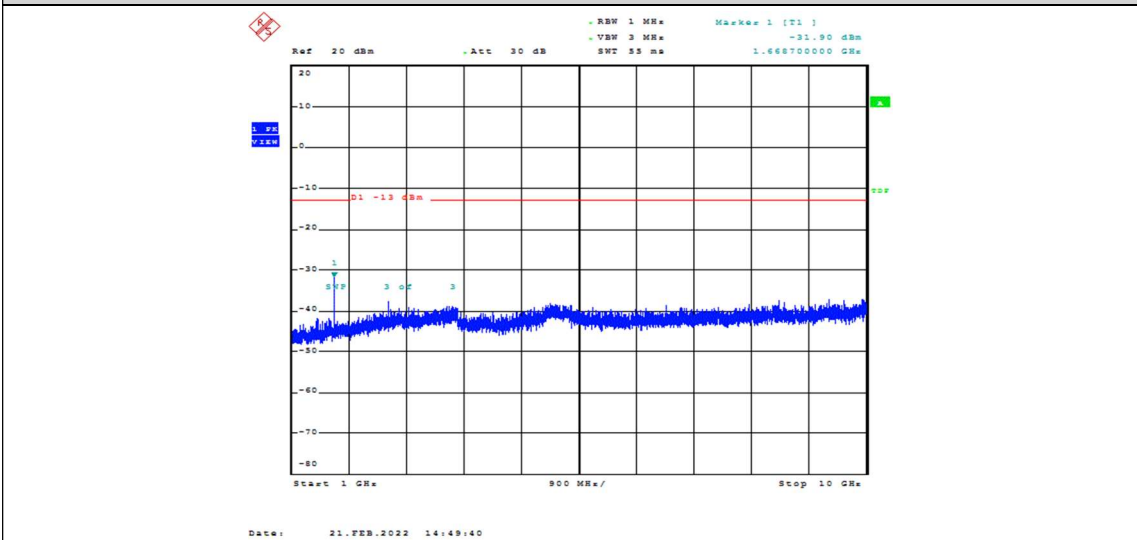
Band26-5MHz-16QAM-26915-1RB#0-Range2:1000~10000MHz
