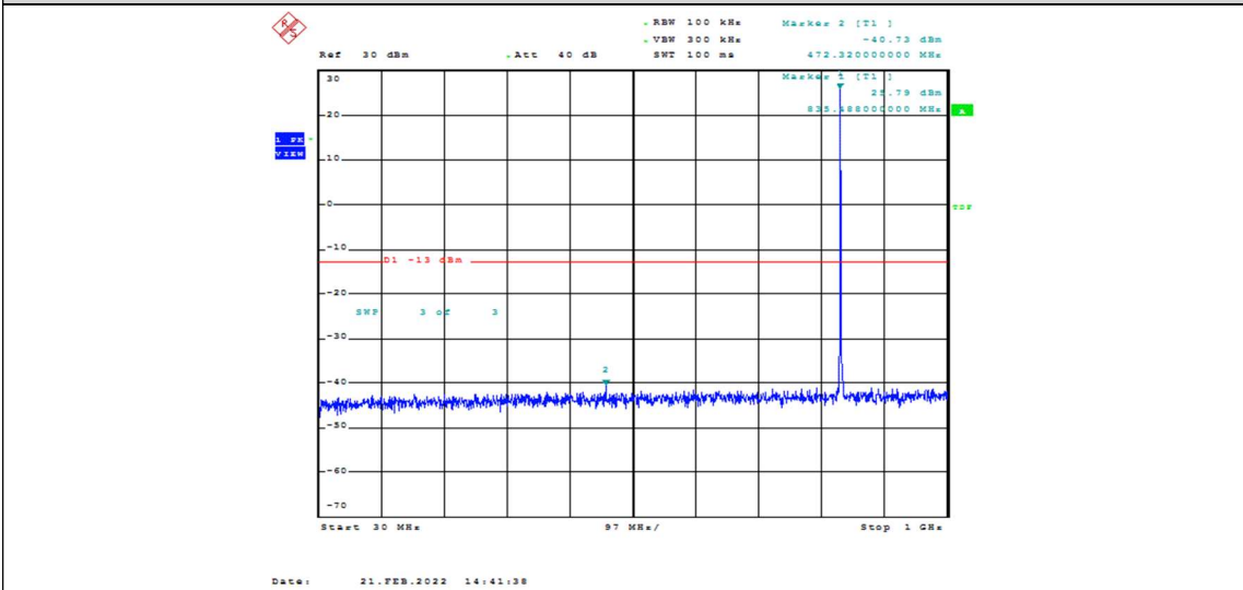
Band26-3MHz-QPSK-26915-1RB#0-Range1:30~1000MHz
