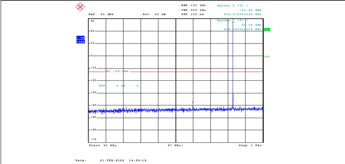
Band26-10MHz-16QAM-26915-1RB#0-Range1: 30~1000MHz
