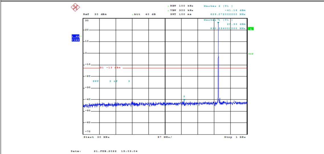
Band26-15MHz-16QAM-26915-1RB#0-Range1: 30~1000MHz
