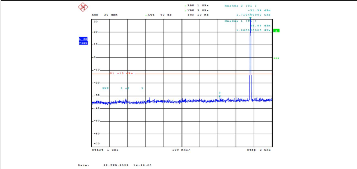
Band2-1.4MHz-QPSK-18900-1RB#0-Range2:1000~2000MHz
