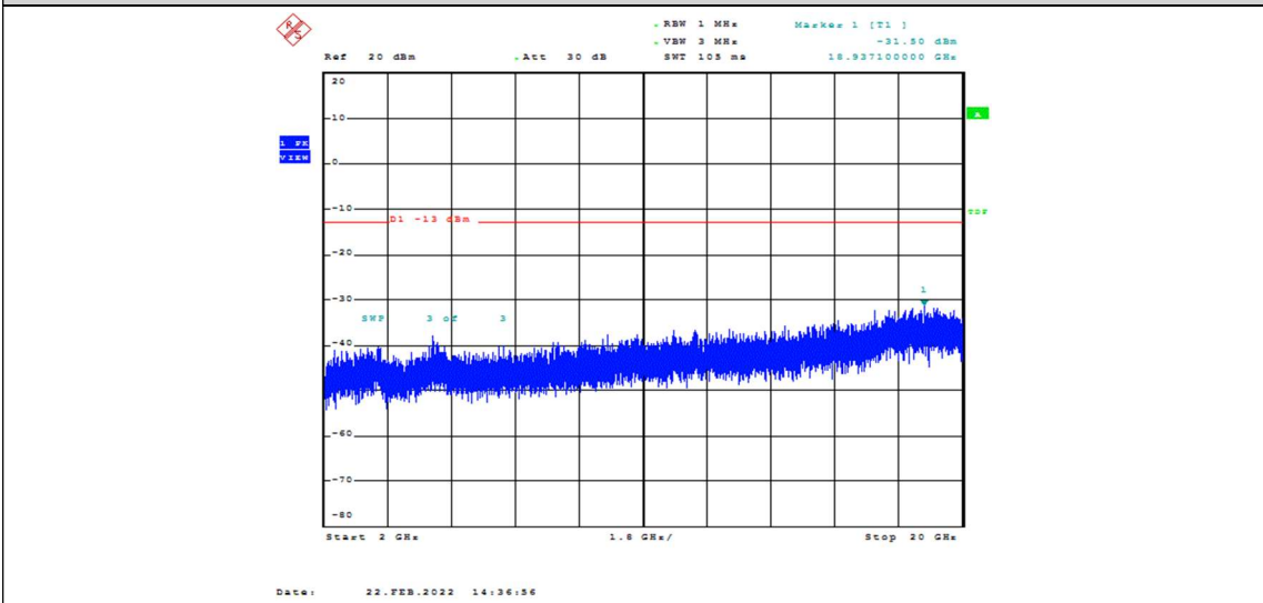
Band2-3MHz-16QAM-18615-1RB#0-Range3:2000~20000MHz
