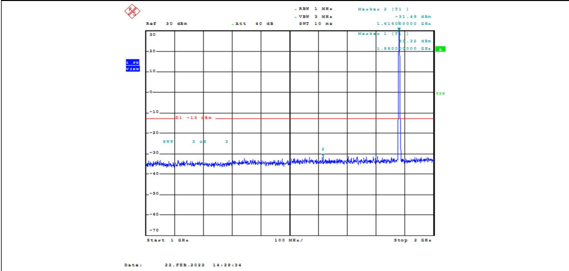
Band2-1.4MHz-16QAM-18900-1RB#0-Range2:1000~2000MHz
