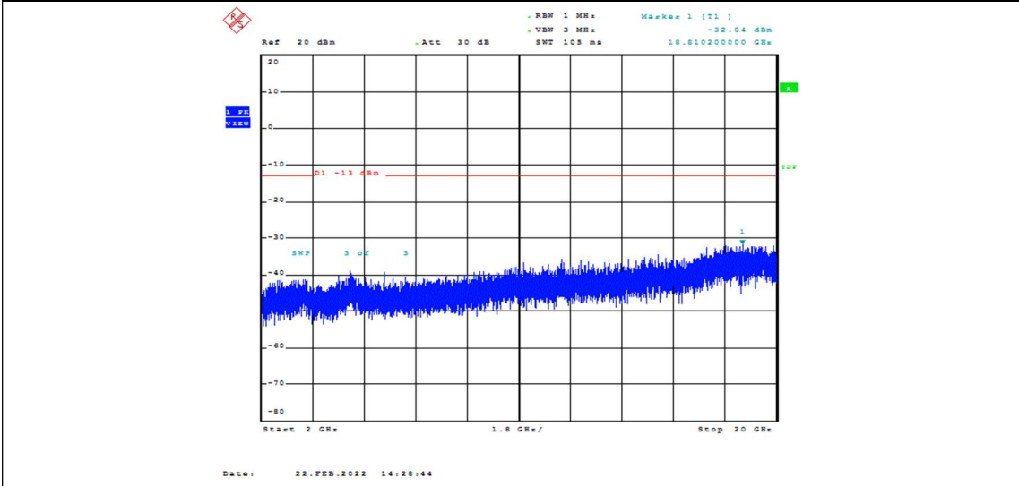
Band2-1.4MHz-16QAM-18900-1RB#0-Range3:2000~20000MHz
