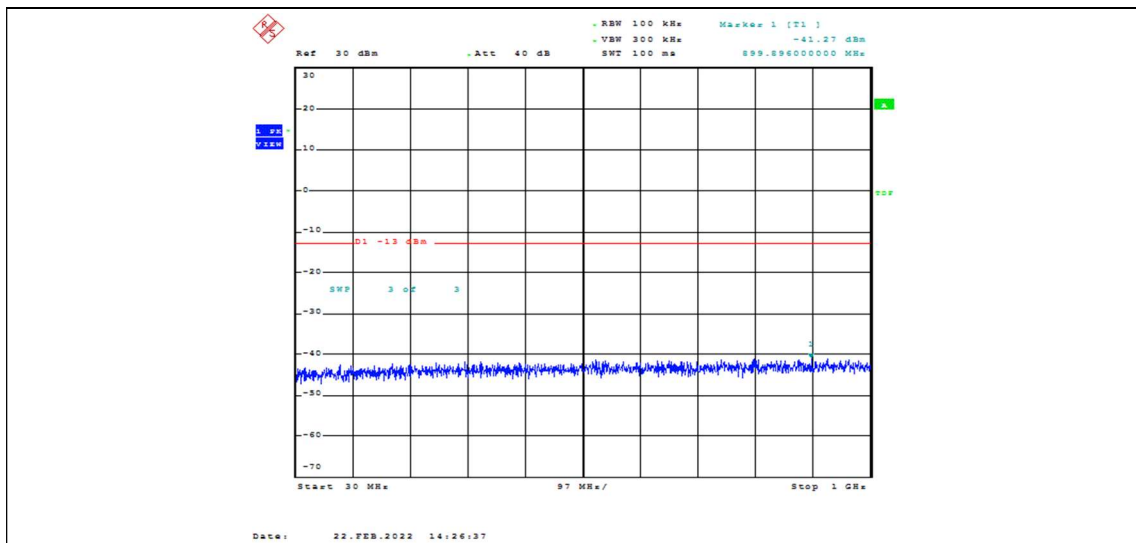
Band2-1.4MHz-QPSK-18607-1RB#0-Range1:30~1000MHz
