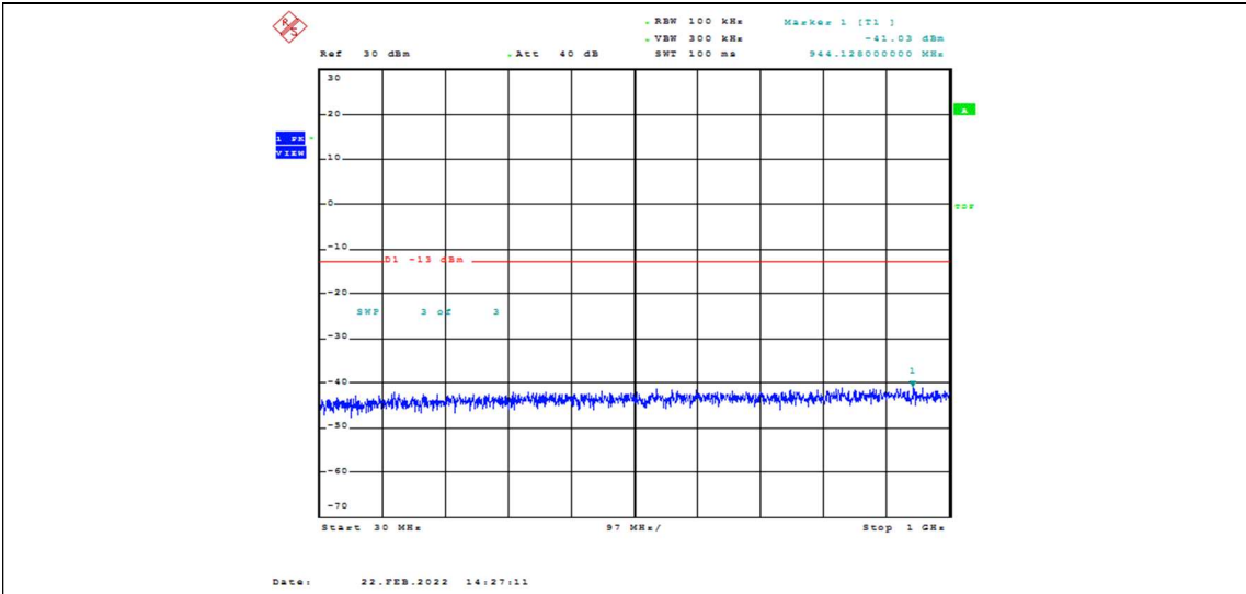
Band2-1.4MHz-16QAM-18607-1RB#0-Range1:30~1000MHz
