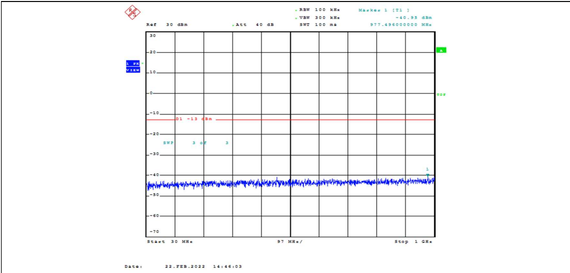
Band2-5MHz-QPSK-18625-1RB#0-Range1:30~1000MHz
