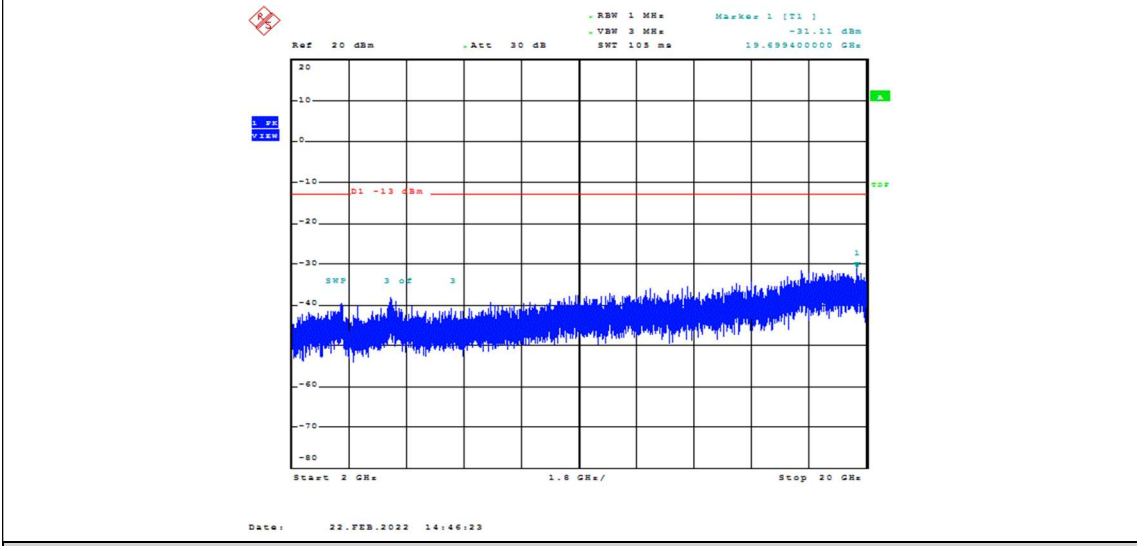
Band2-5MHz-QPSK-18625-1RB#0-Range3:2000~20000MHz
