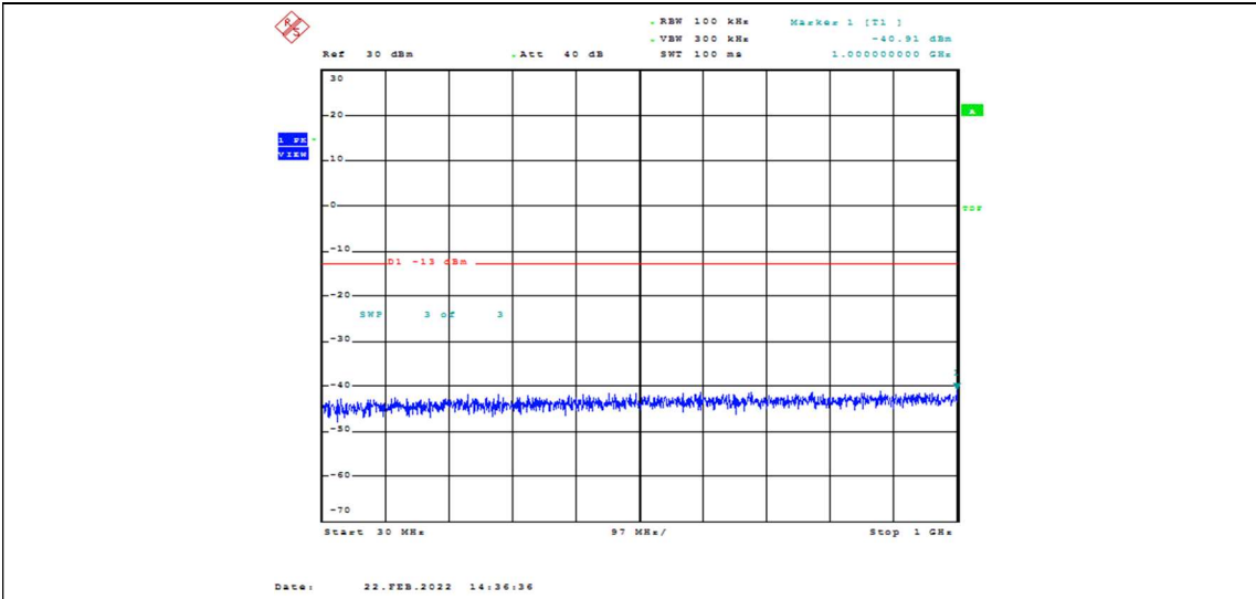
Band2-3MHz-16QAM-18615-1RB#0-Range1:30~1000MHz
