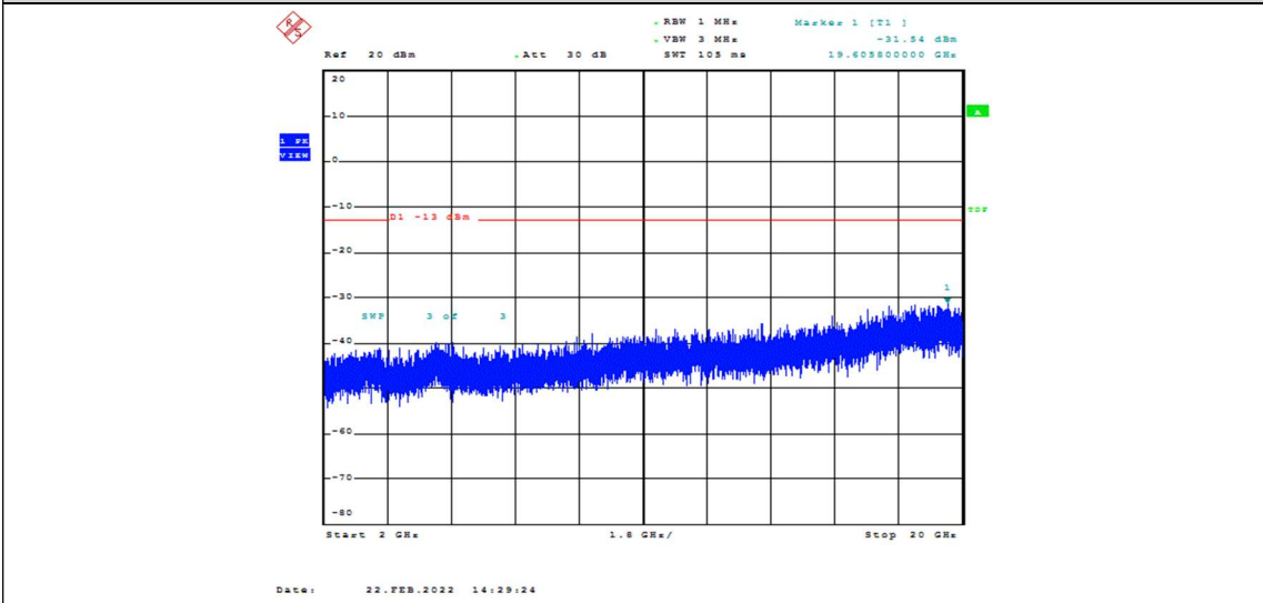
Band2-1.4MHz-QPSK-19193-1RB#0-Range3:2000~20000MHz
