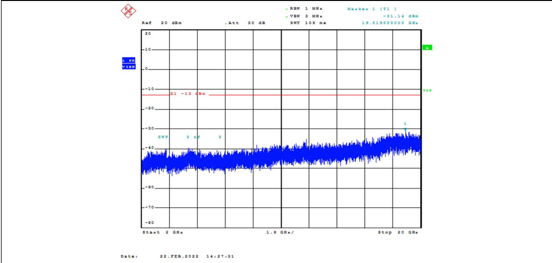
Band2-1.4MHz-16QAM-18607-1RB#0-Range3:2000~20000MHz
