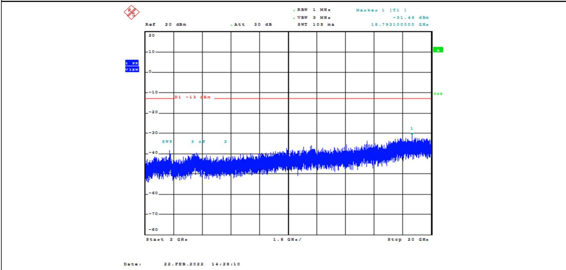
Band2-1.4MHz-QPSK-18900-1RB#0-Range3:2000~20000MHz
