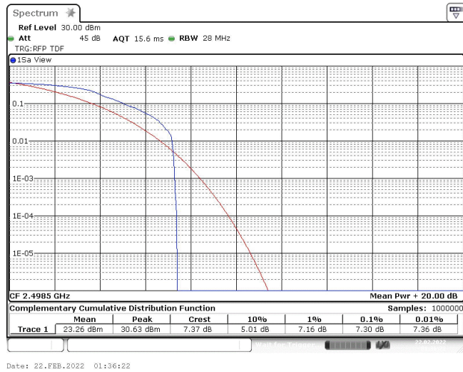
Band41-5MHz-QPSK-39675-1RB#0
