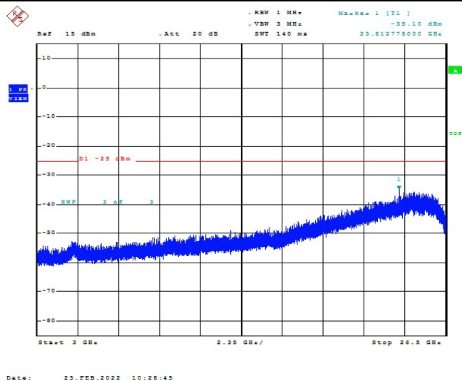
Band41-5MHz-16QAM-40620-1RB#0-Range1:3000~26500MHz
