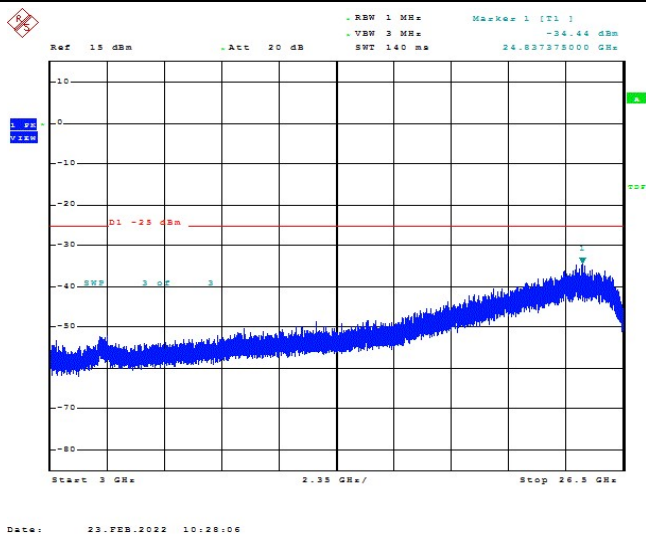
Band41-5MHz-16QAM-39675-1RB#0-Range1:3000~26500MHz
