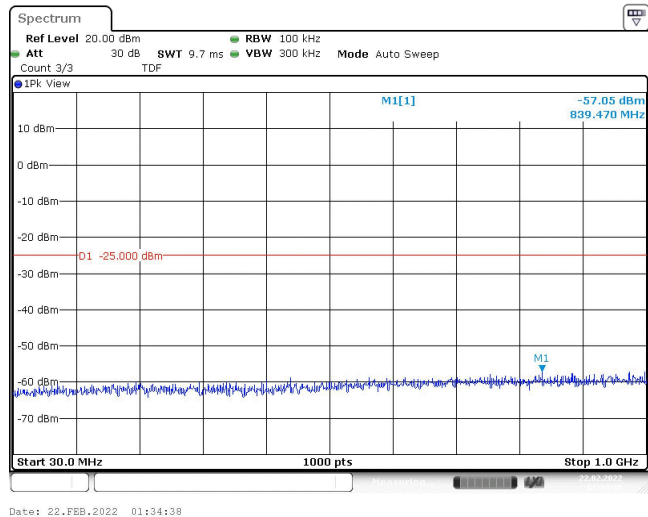
Band41-5MHz-16QAM-40620-1RB#0-Range1:30~1000MHz
