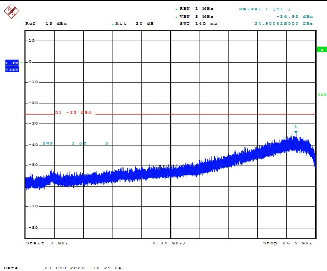
Band41-5MHz-16QAM-41565-1RB#0-Range1:3000~26500MHz
