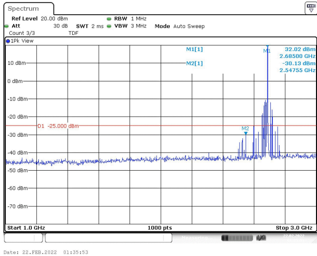
Band41-5MHz-16QAM-41565-1RB#0-Range2:1000~3000MHz
