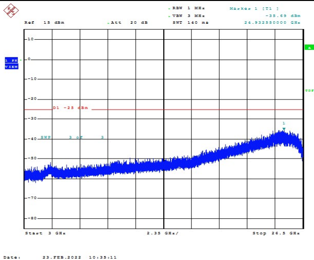
Band41-15MHz-QPSK-39725-1RB#0-Range1:3000~26500MHz
