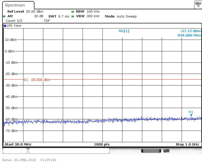
Band41-5MHz-16QAM-41565-1RB#0-Range1:30~1000MHz
