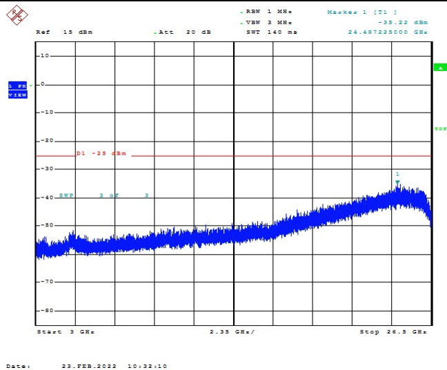
Band41-10MHz-QPSK-40620-1RB#0-Range1:3000~26500MHz
