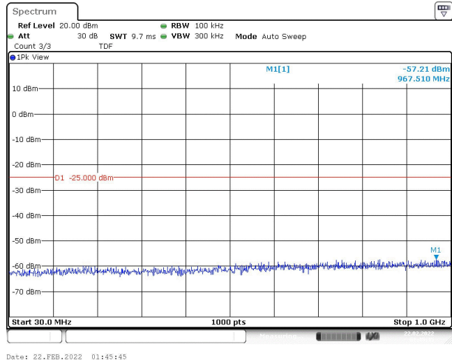
Band41-10MHz-QPSK-40620-1RB#0-Range1:30~1000MHz
