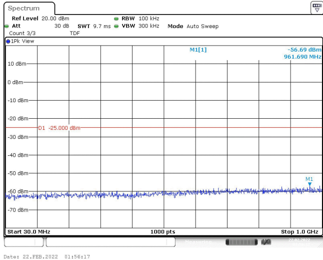
Band41-15MHz-QPSK-39725-1RB#0-Range1:30~1000MHz
