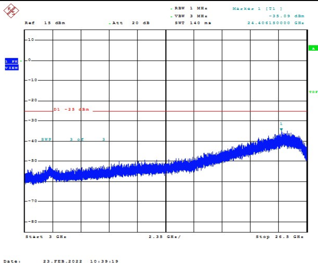
Band41-20MHz-QPSK-40620-1RB#0-Range1:3000~26500MHz
