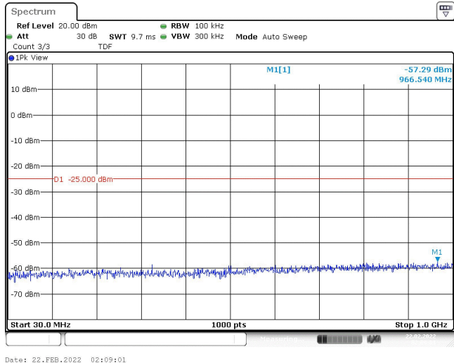
Band41-20MHz-QPSK-40620-1RB#0-Range1:30~1000MHz
