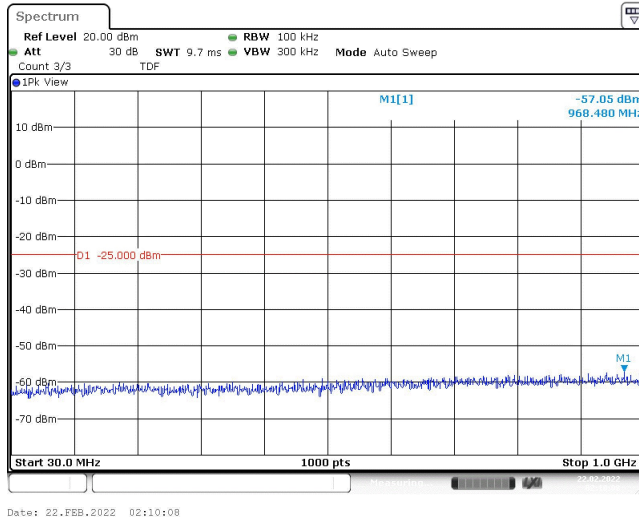
Band41-20MHz-QPSK-41490-1RB#0-Range1:30~1000MHz
