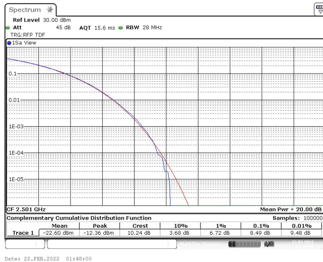
Band41-10MHz-QPSK-39700-1RB#0
