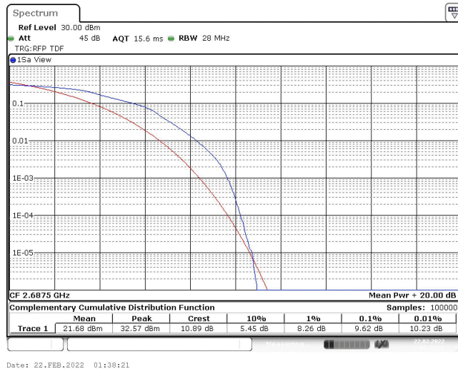
Band41-5MHz-16QAM-41565-25RB#0
