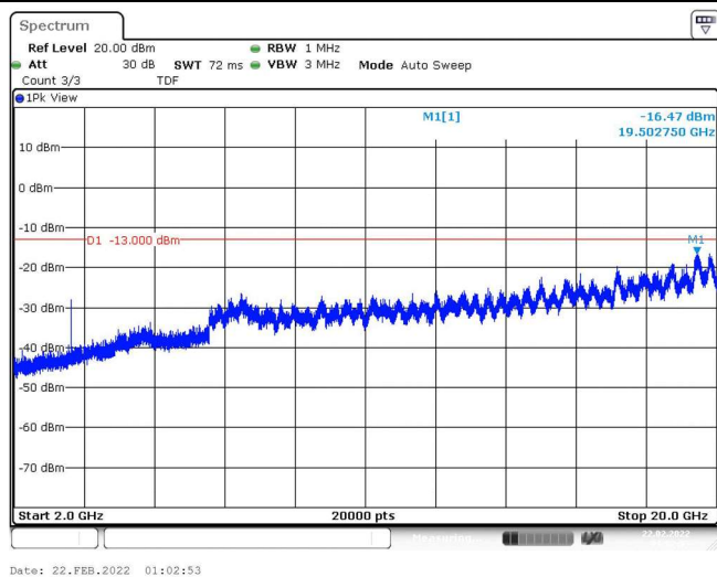
Band4-10MHz-QPSK-20175-1RB#0-Range3:2000~20000MHz
