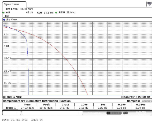
Band5-3MHz-QPSK-20525-1RB#0
