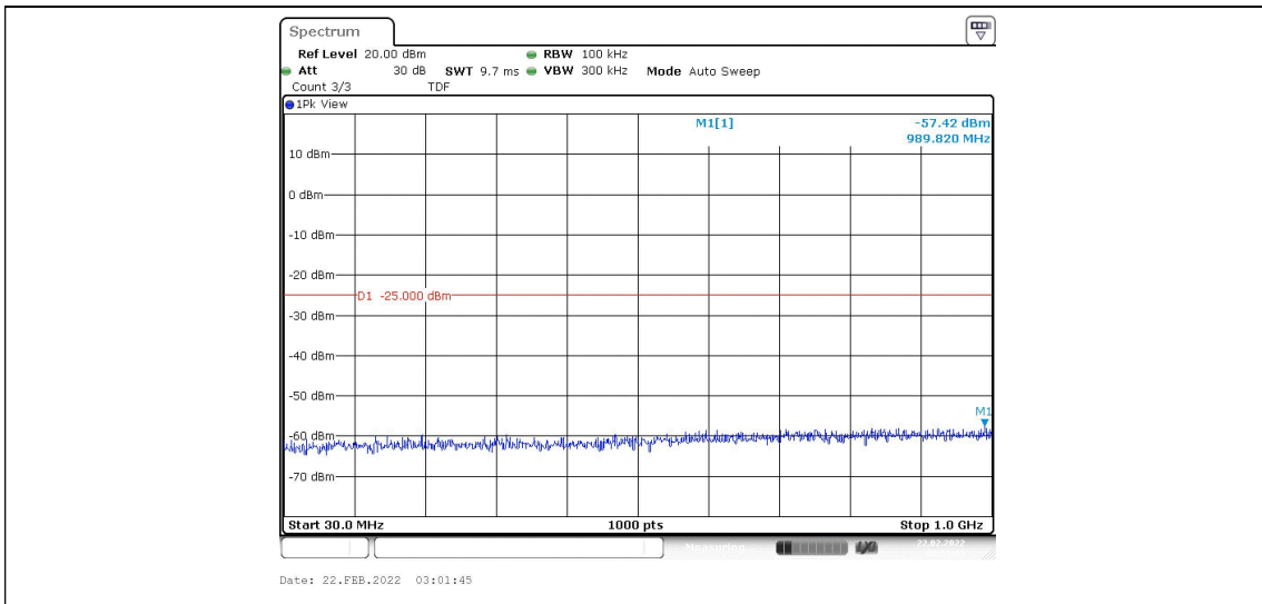
Band7-5MHz-QPSK-20775-1RB#0-Range1:30~1000MHz
