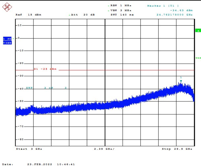
Band7-10MHz-16QAM-21100-1RB#0-Range1:3000~26500MHz
