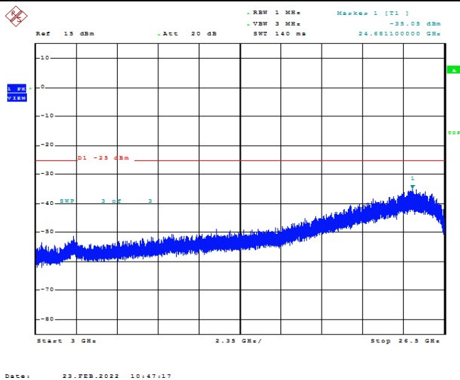
Band7-10MHz-16QAM-21400-1RB#0-Range1:3000~26500MHz
