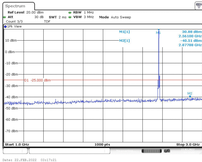
Band7-10MHz-16QAM-21400-1RB#0-Range2:1000~3000MHz
