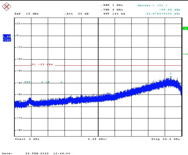
Band7-10MHz-16QAM-20800-1RB#0-Range1:3000~26500MHz
