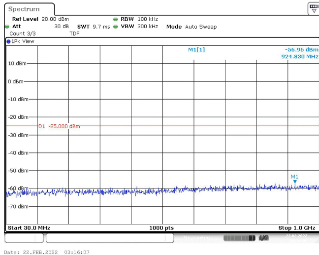
Band7-10MHz-16QAM-21100-1RB#0-Range1:30~1000MHz
