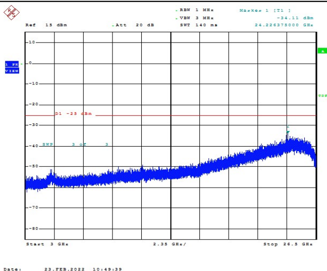
Band7-15MHz-16QAM-20825-1RB#0-Range1:3000~26500MHz
