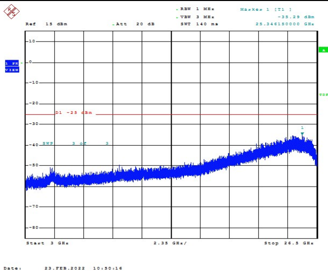
Band7-15MHz-16QAM-21100-1RB#0-Range1:3000~26500MHz
