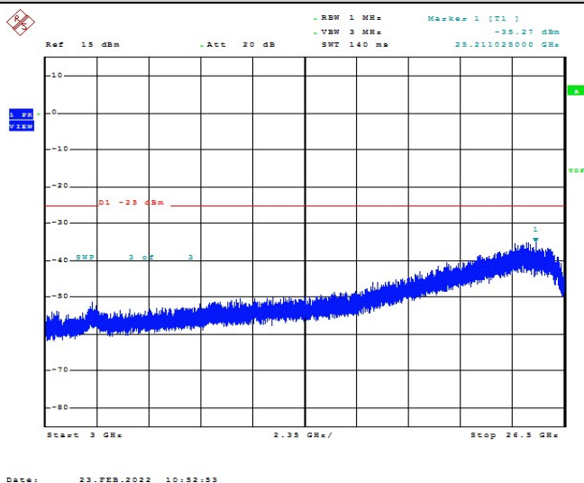
Band7-20MHz-16QAM-20850-1RB#0-Range1:3000~26500MHz
