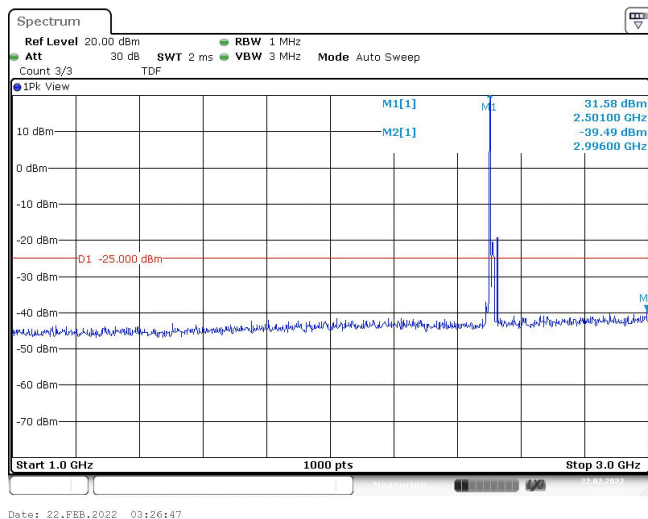
Band7-15MHz-16QAM-20825-1RB#0-Range2:1000~3000MHz
