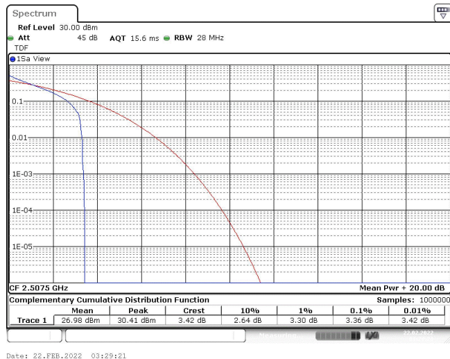
Band7-15MHz-QPSK-20825-1RB#0
