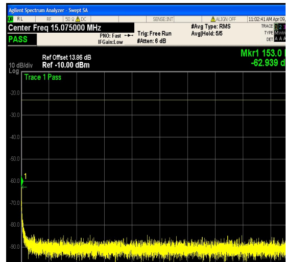
1-N12-PC3-15-5-L-17-CP-QPSK-Edge_1RB _Right-1@24-0.15-30-Ant1--62.94--23-PASS
