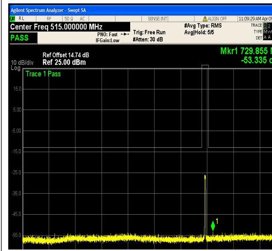
1-N12-PC3-15-5-L-21-CP-16QAM-Outer_Full -25@0-30-1000-Ant1--53.34--13-PASS
