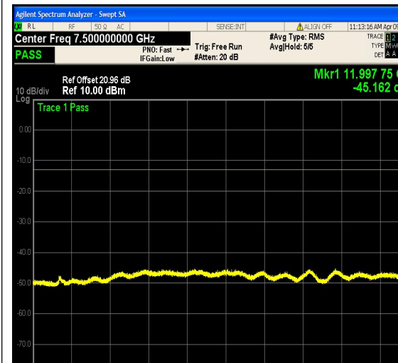
1-N12-PC3-15-5-L-23-CP-64QAM-Edge_1R B_Right-1@24-3000-12000-Ant1--45.16--13- PASS
