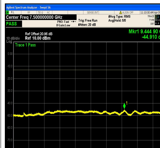
1-N12-PC3-15-5-L-21-CP-16QAM-Outer_Full
