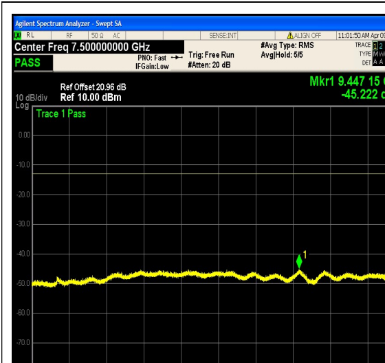
1-N12-PC3-15-5-L-16-CP-QPSK-Edge_1RB _Left-1@0-3000-12000-Ant1--45.22--13-PAS S
