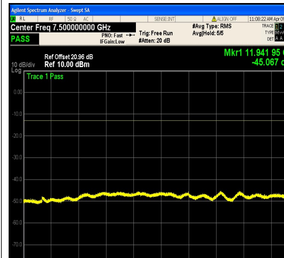
1-N12-PC3-15-5-L-20-CP-16QAM-Edge_1R B_Right-1@24-3000-12000-Ant1--45.07--13- PASS
