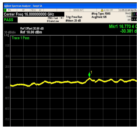
1-N12-PC3-15-5-L-18-CP-QPSK-Outer_Full-
