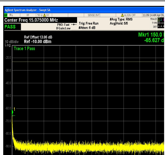
1-N12-PC3-15-5-L-21-CP-16QAM-Outer_Full -25@0-0.15-30-Ant1--65.63--23-PASS
