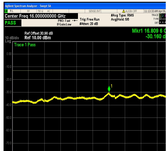
1-N12-PC3-15-5-L-23-CP-64QAM-Edge_1R B_Right-1@24-12000-20000-Ant1--30.16--13 -PASS
