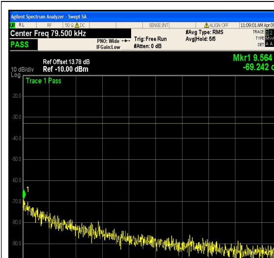
1-N12-PC3-15-5-L-21-CP-16QAM-Outer_Full -25@0-0.009-0.15-Ant1--69.24--33-PASS
