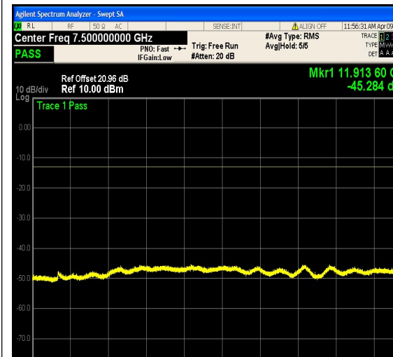
1-N12-PC3-15-5-M-20-CP-16QAM-Edge_1R B_Right-1@24-3000-12000-Ant1--45.28--13- PASS
