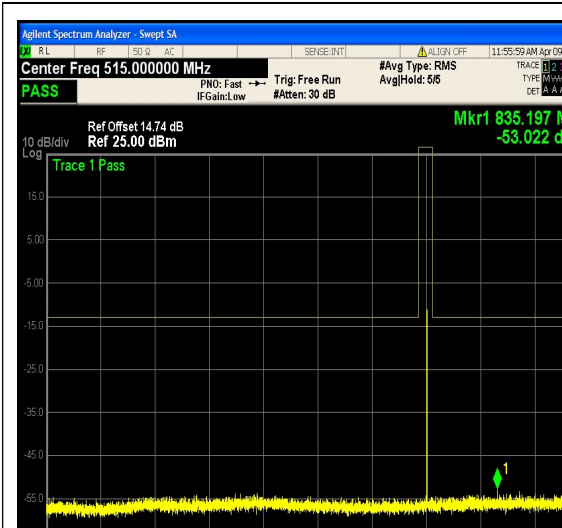
1-N12-PC3-15-5-M-20-CP-16QAM-Edge_1R B_Right-1@24-30-1000-Ant1--53.02--13-PAS S
