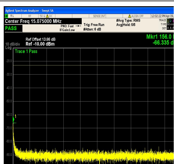
1-N12-PC3-15-5-M-24-CP-64QAM-Outer_Ful I-25@0-0.15-30-Ant1--66.33--23-PASS
