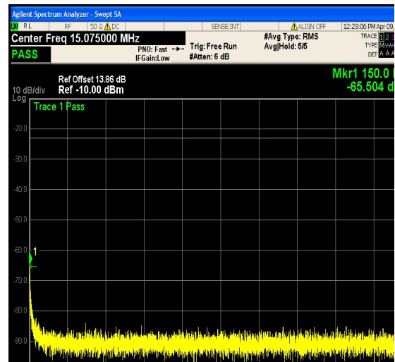
1-N12-PC3-15-5-H-8-DFT-16QAM-Edge_1R B_Right-1@24-0.15-30-Ant1--65.50--23-PAS S
