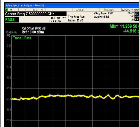
1-N12-PC3-15-5-H-17-CP-QPSK-Edge_1RB _Right-1@24-3000-12000-Ant1--44.92--13-PASS
