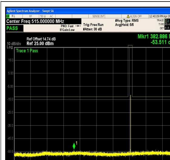
1-N12-PC3-15-5-H-17-CP-QPSK-Edge_1RB _Right-1@24-30-1000-Ant1--53.51--13-PASS
