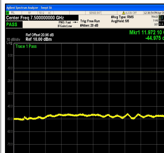
1-N12-PC3-15-5-H-15-DFT-256QAM-Outer_
