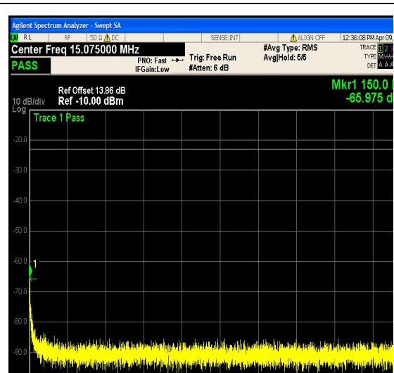
1-N12-PC3-15-5-H-15-DFT-256QAM-Outer_ Full-25@0-0.15-30-Ant1--65.97--23-PASS
