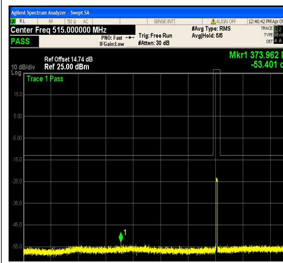
1-N12-PC3-15-5-H-21-CP-16QAM-Outer_Ful I-25@0-30-1000-Ant1--53.40--13-PASS
