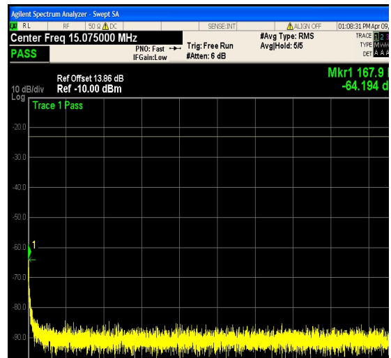
1-N12-PC3-15-10-L-5-DFT-QPSK-Edge_1RB _Right-1@51-0.15-30-Ant1--64.19--23-PASS
