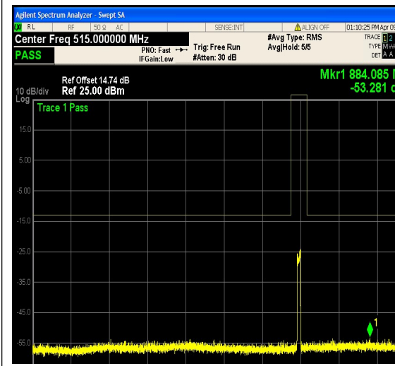
1-N12-PC3-15-10-L-6-DFT-QPSK-Outer_Full -50@0-30-1000-Ant1--53.28--13-PASS
