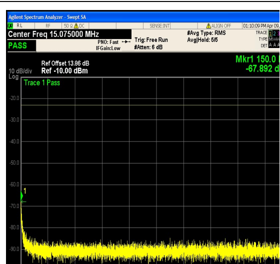
1-N12-PC3-15-10-L-6-DFT-QPSK-Outer_Full -50@0-0.15-30-Ant1--67.89--23-PASS
