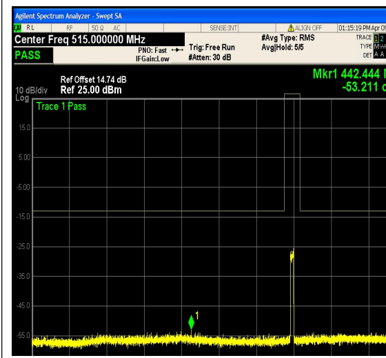
1-N12-PC3-15-10-L-9-DFT-16QAM-Outer_Fu II-50@0-30-1000-Ant1--53.21--13-PASS
