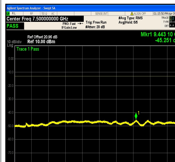
1-N12-PC3-15-10-L-9-DFT-16QAM-Outer_Fu
