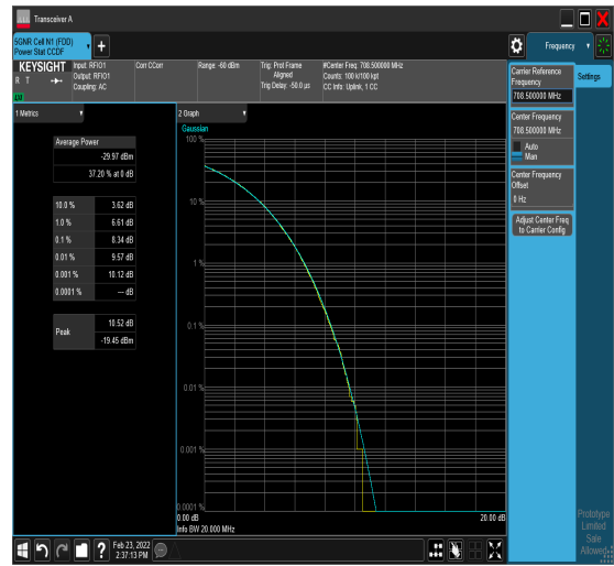
1-N12-PC3-15-15-H-4-DFT-64QAM-Outer_F ull-75@0-8.34-100%-0.00-8.34-PASS-≤13
