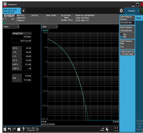
1-N12-PC3-15-15-H-3-DFT-16QAM-Outer_F ull-75@0-8.46-100%-0.00-8.46-PASS-≤13
