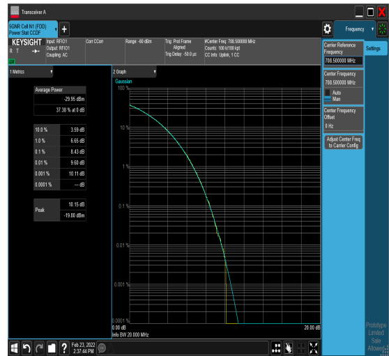
1-N12-PC3-15-15-H-6-CP-QPSK-Outer_Full- 79@0-8.43-100%-0.00-8.43-PASS-≤13
