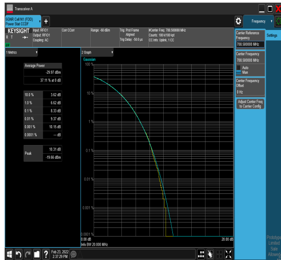
1-N12-PC3-15-15-H-5-DFT-256QAM-Outer_ Full-75@0-8.33-100%-0.00-8.33-PASS-≤13
