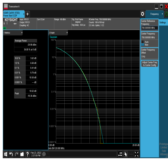
1-N12-PC3-15-15-H-5-DFT-256QAM-Outer_ Full-75@0-8.33-100%-0.00-8.33-PASS-≤13
