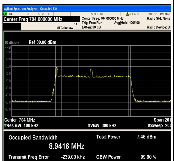
1-N12-PC3-15-10-L-2-DFT-PI2BPSK-Outer_Full
