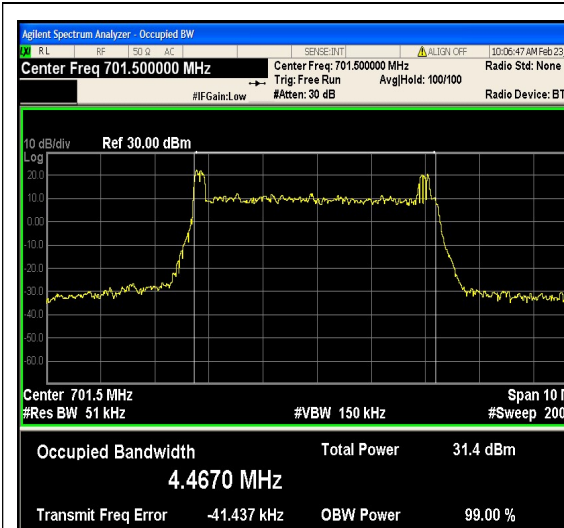
1-N12-PC3-15-5-L-5-CP-QPSK-Outer_Full-2 5@0-Ant1-4.4670-4.658-≤5-PASS
