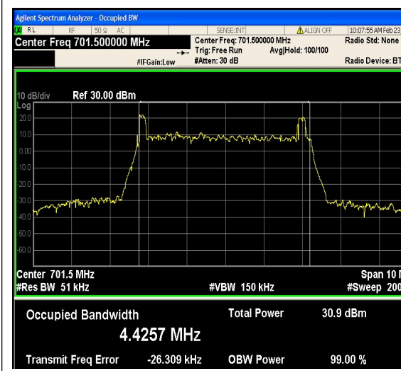
1-N12-PC3-15-5-L-7-CP-64QAM-Outer_Full-25@0-Ant1-4.4257-4.657-≤5-PASS
