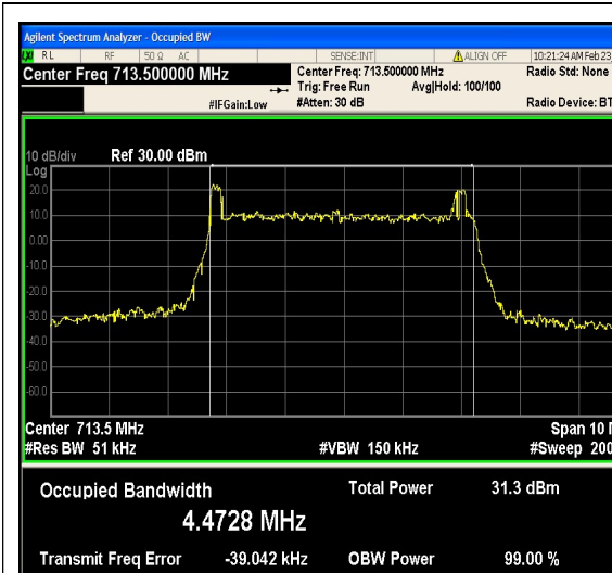
1-N12-PC3-15-5-H-5-CP-QPSK-Outer_Full-2 5@0-Ant1-4.4728-4.663-≤5-PASS
