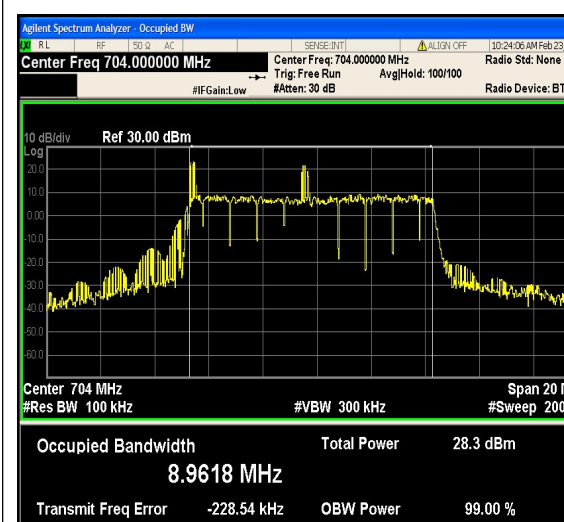
1-N12-PC3-15-10-L-1-DFT-QPSK-Outer_Full
