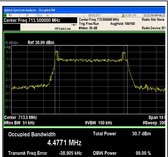
1-N12-PC3-15-5-H-6-CP-16QAM-Outer_Full-25@0-Ant1-4.4771-4.669-≤5-PASS
