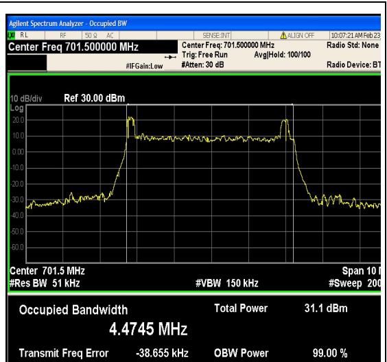
1-N12-PC3-15-5-L-6-CP-16QAM-Outer_Full-25@0-Ant1-4.4745-4.656-≤5-PASS
