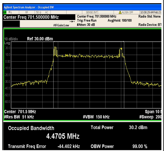
1-N12-PC3-15-5-L-8-CP-256QAM-Outer_Full-25@0-Ant1-4.4705-4.647-≤5-PASS
