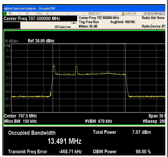
1-N12-PC3-15-15-M-2-DFT-PI2BPSK-Outer_Full-79@0-Ant1-13.491-14.06-≤15-PASS
