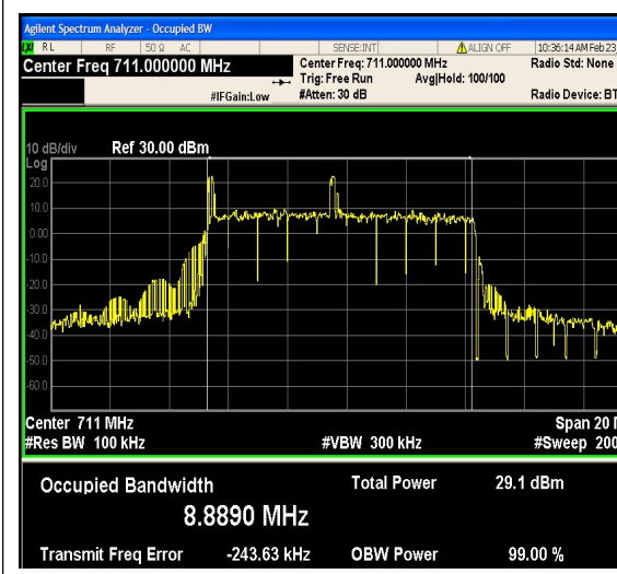
1-N12-PC3-15-10-H-1-DFT-QPSK-Outer_Full
