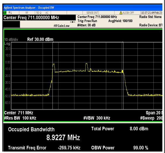
1-N12-PC3-15-10-H-2-DFT-PI2BPSK-Outer_Full
