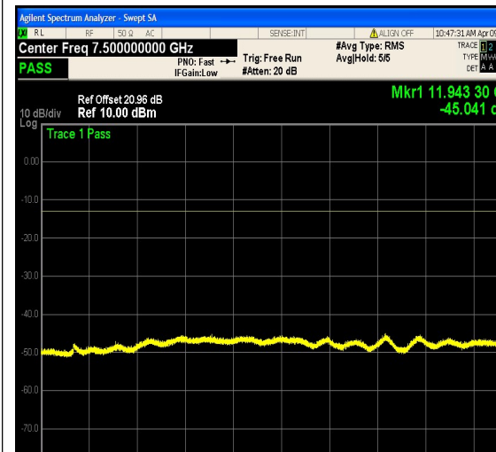
1-N12-PC3-15-5-L-8-DFT-16QAM-Edge_1R B_Right-1@24-3000-12000-Ant1--45.04--13- PASS
