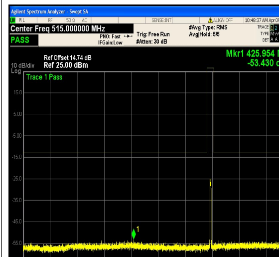
1-N12-PC3-15-5-L-9-DFT-16QAM-Outer_Full -25@0-30-1000-Ant1--53.43--13-PASS
