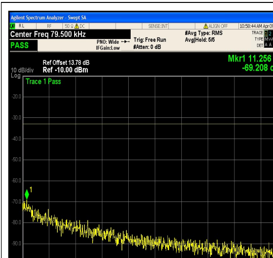
1-N12-PC3-15-5-L-15-DFT-256QAM-Outer_F ull-25@0-0.009-0.15-Ant1--69.21--33-PASS
