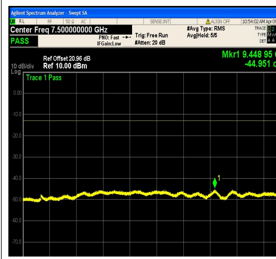
1-N12-PC3-15-5-L-12-DFT-64QAM-Outer_Fu
