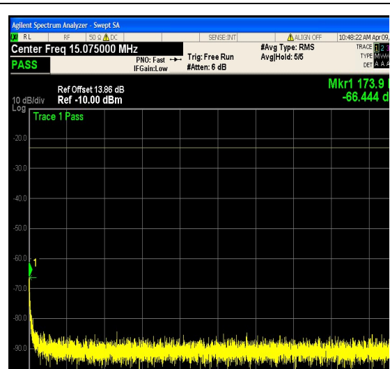
1-N12-PC3-15-5-L-9-DFT-16QAM-Outer_Full -25@0-0.15-30-Ant1--66.44--23-PASS
