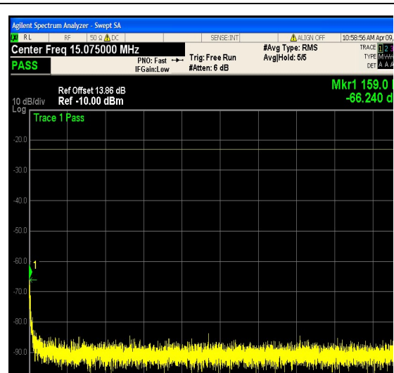
1-N12-PC3-15-5-L-15-DFT-256QAM-Outer_F ull-25@0-0.15-30-Ant1--66.24--23-PASS
