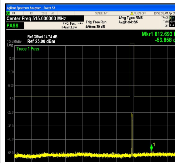
1-N12-PC3-15-5-L-12-DFT-64QAM-Outer_Fu Il-25@0-30-1000-Ant1--53.86--13-PASS
