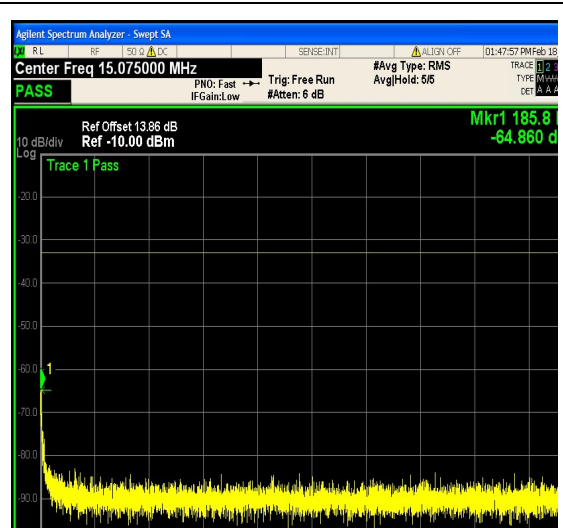
1-N25-PC3-15-5-L-9-DFT-16QAM-Outer_Full -25@0-0.15-30-Ant1--64.86--33-PASS
