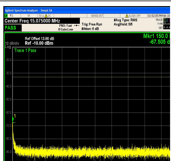
1-N25-PC3-15-5-L-12-DFT-64QAM-Outer_Fu Il-25@0-0.15-30-Ant1--67.51--33-PASS
