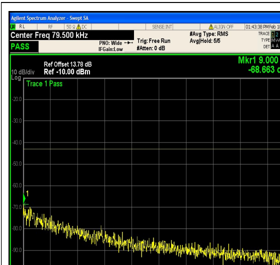
1-N25-PC3-15-5-L-6-DFT-QPSK-Outer_Full- 25@0-0.009-0.15-Ant1--68.66--43-PASS
