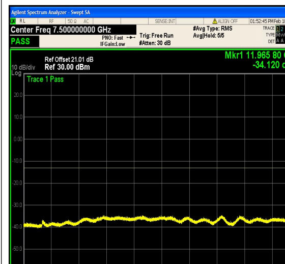
1-N25-PC3-15-5-L-12-DFT-64QAM-Outer_Fu
