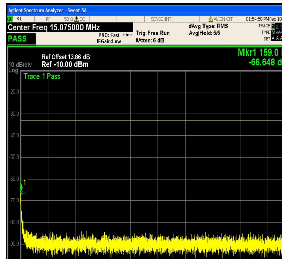
1-N25-PC3-15-5-L-14-DFT-256QAM-Edge_1 RB_Right-1@24-0.15-30-Ant1--66.65--33-PA SS
