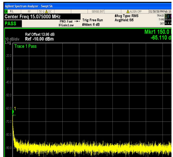
1-N25-PC3-15-5-L-17-CP-QPSK-Edge_1RB _Right-1@24-0.15-30-Ant1--65.11--33-PASS
