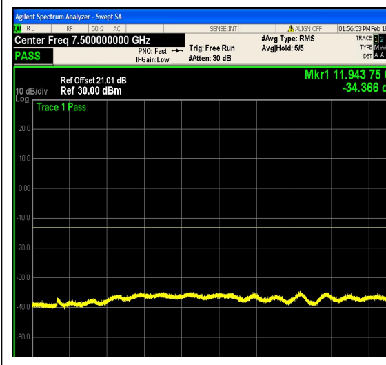
1-N25-PC3-15-5-L-15-DFT-256QAM-Outer_F
