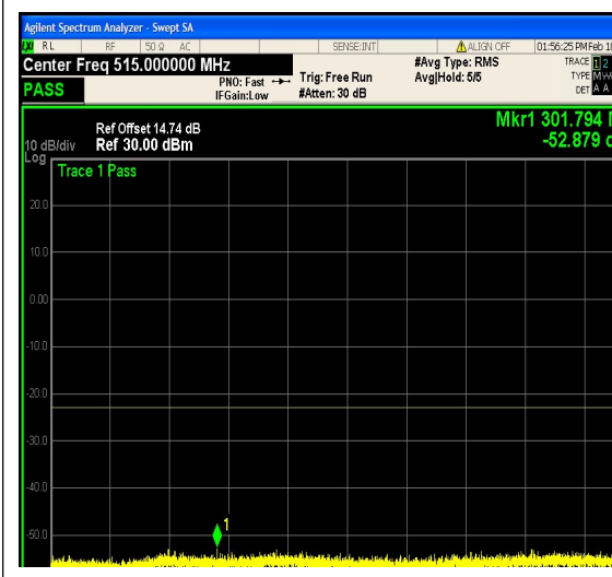
1-N25-PC3-15-5-L-15-DFT-256QAM-Outer_F ull-25@0-30-1000-Ant1--52.88--23-PASS
