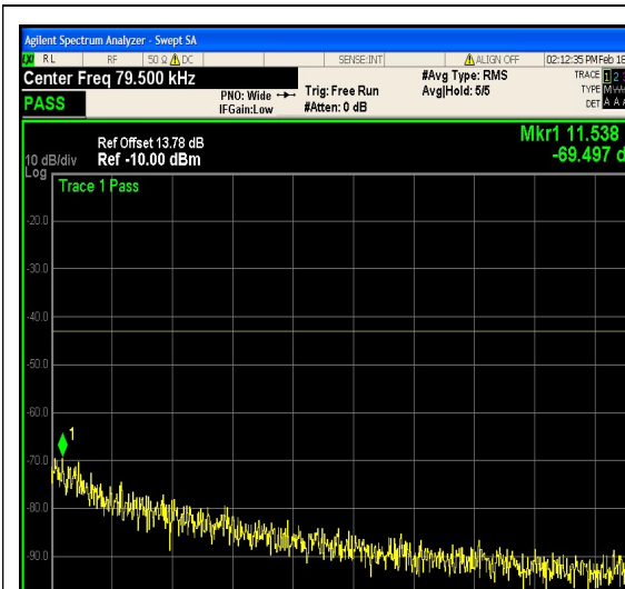
1-N25-PC3-15-5-L-27-CP-256QAM-Outer_F ull-25@0-0.009-0.15-Ant1--69.50--43-PASS
