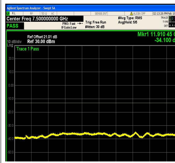
1-N25-PC3-15-5-L-27-CP-256QAM-Outer_F
