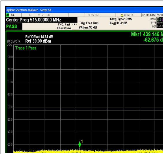
1-N25-PC3-15-5-L-26-CP-256QAM-Edge_1R B_Right-1@24-30-1000-Ant1--52.68--23-PAS S
