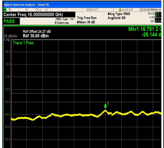
1-N25-PC3-15-5-L-20-CP-16QAM-Edge_1R B_Right-1@24-12000-20000-Ant1--26.14--13 -PASS
