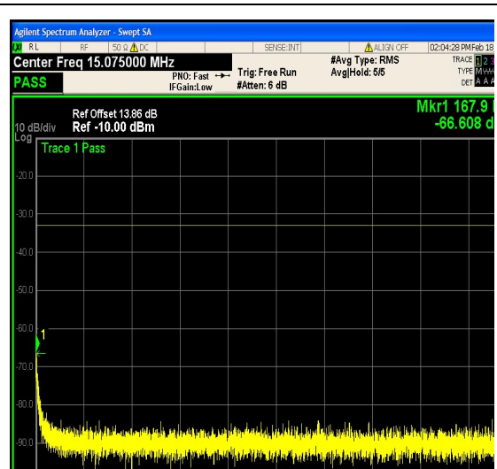
1-N25-PC3-15-5-L-21-CP-16QAM-Outer_Full -25@0-0.15-30-Ant1--66.61--33-PASS
