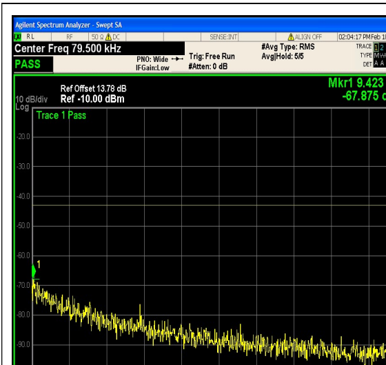
1-N25-PC3-15-5-L-21-CP-16QAM-Outer_Full -25@0-0.009-0.15-Ant1--67.87--43-PASS
