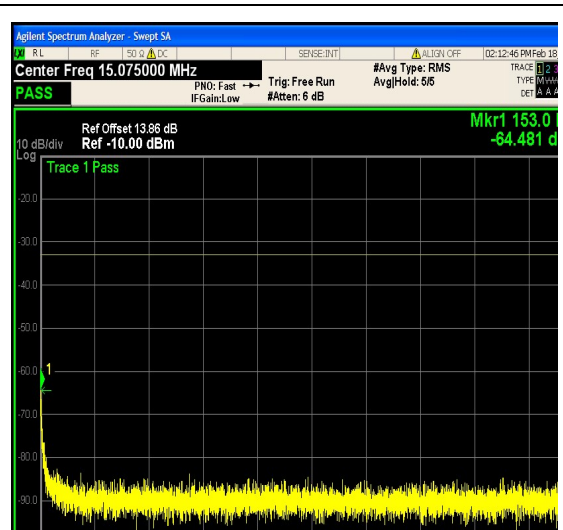
1-N25-PC3-15-5-L-27-CP-256QAM-Outer_F ull-25@0-0.15-30-Ant1--64.48--33-PASS
