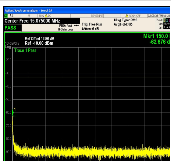
1-N25-PC3-15-5-L-24-CP-64QAM-Outer_Full -25@0-0.15-30-Ant1--62.68--33-PASS
