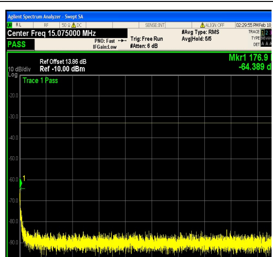
1-N25-PC3-15-5-M-12-DFT-64QAM-Outer_F ull-25@0-0.15-30-Ant1--64.39--33-PASS
