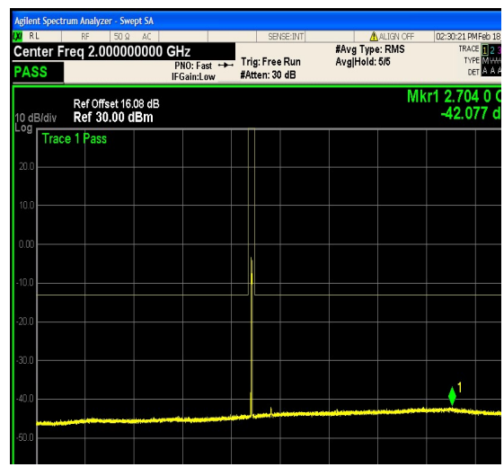
1-N25-PC3-15-5-M-12-DFT-64QAM-Outer_F ull-25@0-1000-3000-Ant1--42.08--13-PASS
