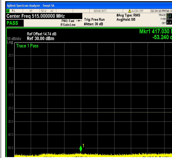
1-N25-PC3-15-5-M-15-DFT-256QAM-Outer_ Full-25@0-30-1000-Ant1--53.24--23-PASS
