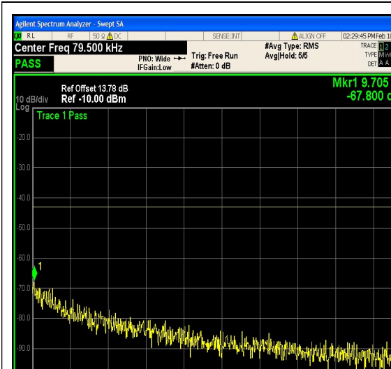
1-N25-PC3-15-5-M-12-DFT-64QAM-Outer_F ull-25@0-0.009-0.15-Ant1--67.80--43-PASS
