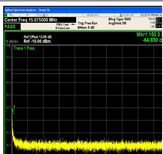
1-N25-PC3-15-5-M-9-DFT-16QAM-Outer_Ful I-25@0-0.15-30-Ant1--64.83--33-PASS
