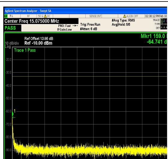
1-N25-PC3-15-5-M-18-CP-QPSK-Outer_Full- 25@0-0.15-30-Ant1--64.74--33-PASS
