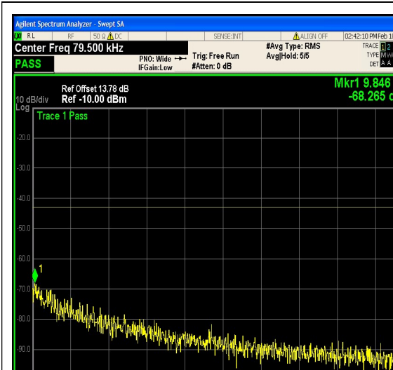
1-N25-PC3-15-5-M-21-CP-16QAM-Outer_Ful I-25@0-0.009-0.15-Ant1--68.26--43-PASS
