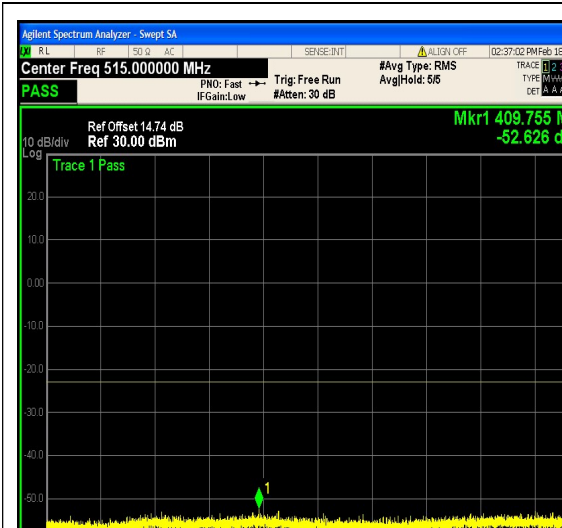
1-N25-PC3-15-5-M-17-CP-QPSK-Edge_1RB _Right-1@24-30-1000-Ant1--52.63--23-PASS
