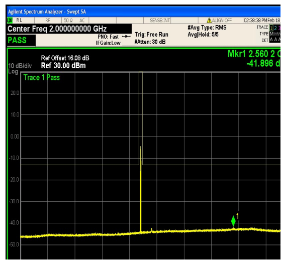
1-N25-PC3-15-5-M-18-CP-QPSK-Outer_Full- 25@0-1000-3000-Ant1--41.90--13-PASS
