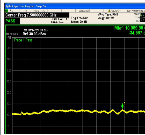
1-N25-PC3-15-5-M-24-CP-64QAM-Outer_Ful
