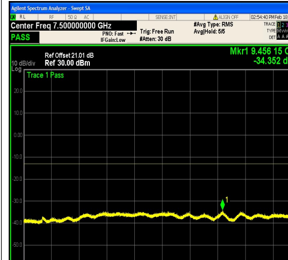
1-N25-PC3-15-5-H-2-DFT-PI2BPSK-Edge_1 RB_Right-1@24-3000-12000-Ant1--34.35--1 3-PASS
