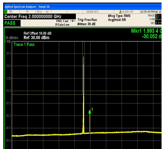
1-N25-PC3-15-5-H-3-DFT-PI2BPSK-Outer_F ull-25@0-1000-3000-Ant1--30.05--13-PASS
