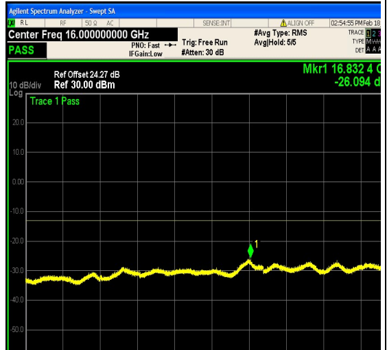
1-N25-PC3-15-5-H-2-DFT-PI2BPSK-Edge_1 RB_Right-1@24-12000-20000-Ant1--26.09-- 13-PASS
