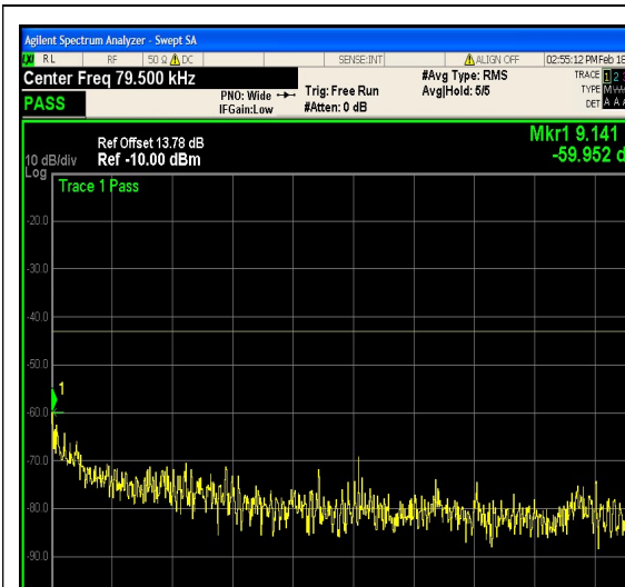
1-N25-PC3-15-5-H-3-DFT-PI2BPSK-Outer_F ull-25@0-0.009-0.15-Ant1--59.95--43-PASS
