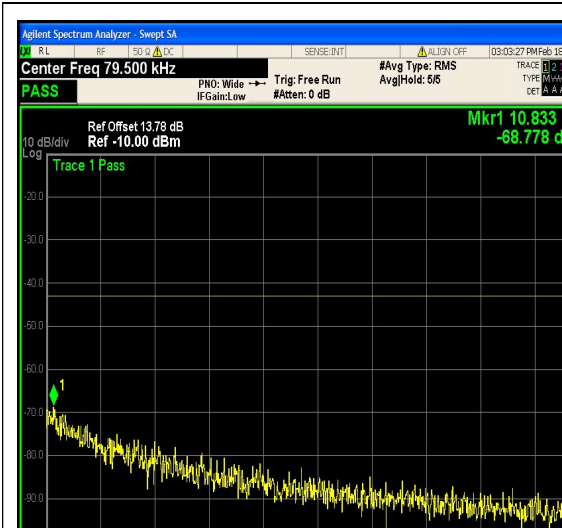
1-N25-PC3-15-5-H-9-DFT-16QAM-Outer_Ful I-25@0-0.009-0.15-Ant1--68.78--43-PASS
