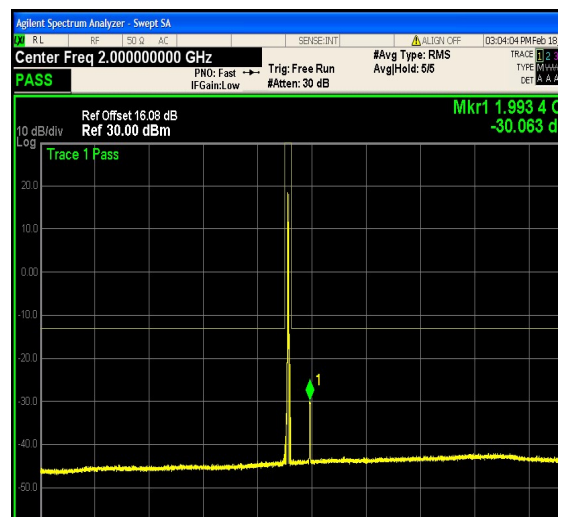
1-N25-PC3-15-5-H-9-DFT-16QAM-Outer_Ful I-25@0-1000-3000-Ant1--30.06--13-PASS
