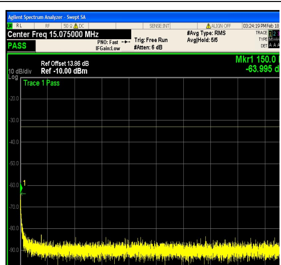
1-N25-PC3-15-5-H-24-CP-64QAM-Outer_Ful I-25@0-0.15-30-Ant1--63.99--33-PASS
