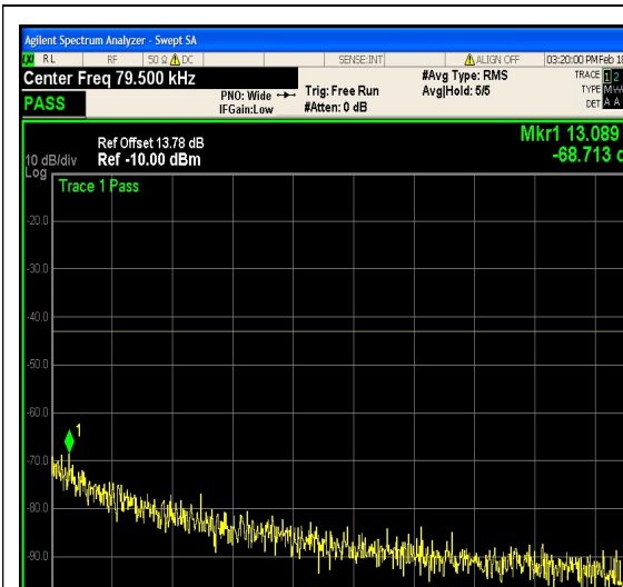
1-N25-PC3-15-5-H-21-CP-16QAM-Outer_Ful I-25@0-0.009-0.15-Ant1--68.71--43-PASS
