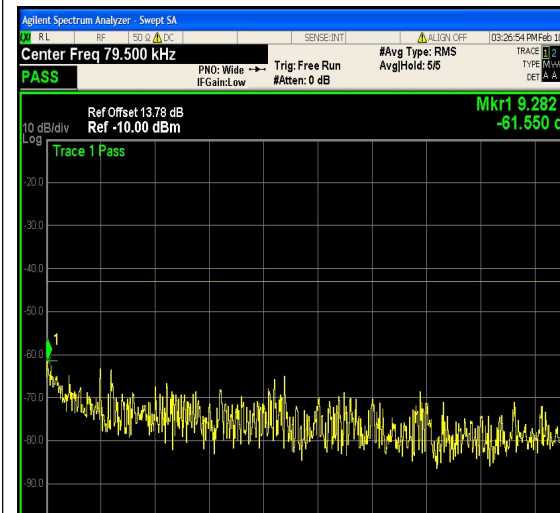
1-N25-PC3-15-5-H-26-CP-256QAM-Edge_1 RB_Right-1@24-0.009-0.15-Ant1--61.55--43- PASS
