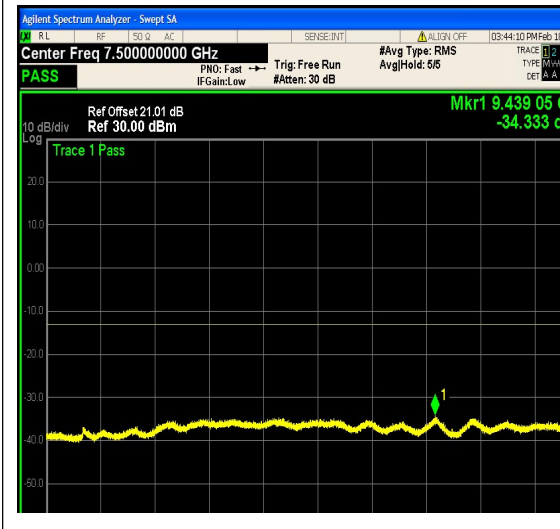
1-N25-PC3-15-10-L-6-DFT-QPSK-Outer_Full
