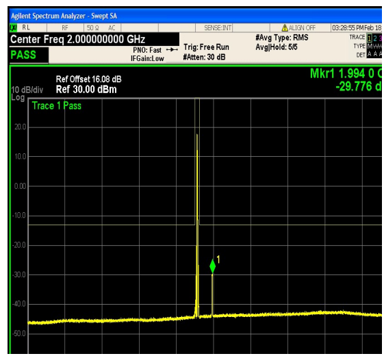
1-N25-PC3-15-5-H-27-CP-256QAM-Outer_F ull-25@0-1000-3000-Ant1--29.78--13-PASS
