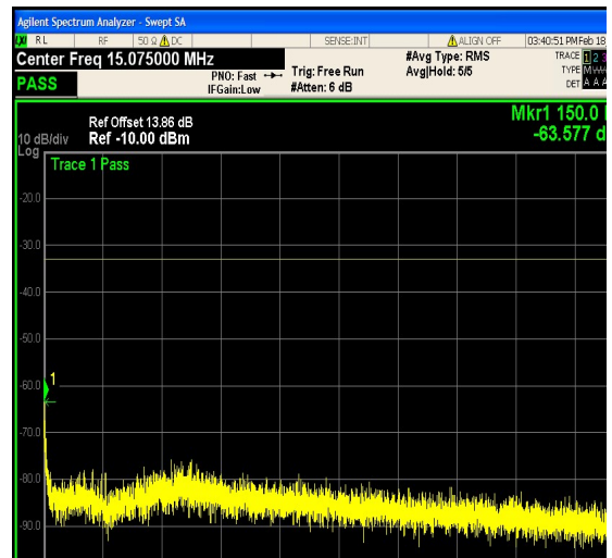
1-N25-PC3-15-10-L-5-DFT-QPSK-Edge_1RB _Right-1@51-0.15-30-Ant1--63.58--33-PASS
