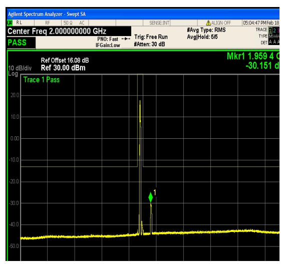
1-N25-PC3-15-10-M-18-CP-QPSK-Outer_Ful l-52@0-0.15-30-Ant1--65.14--33-PASS
