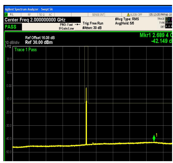
1-N25-PC3-15-10-M-24-CP-64QAM-Outer_F ull-52@0-0.15-30-Ant1--65.94--33-PASS
