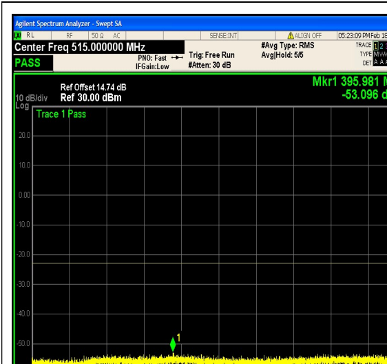
1-N25-PC3-15-10-H-4-DFT-QPSK-Edge_1R B_Left-1@0-30-1000-Ant1--53.10--23-PASS
