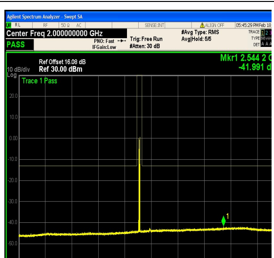
1-N25-PC3-15-10-H-20-CP-16QAM-Edge_1 RB_Right-1@51-1000-3000-Ant1--41.99--13- PASS
