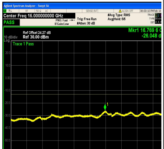
1-N25-PC3-15-15-L-2-DFT-PI2BPSK-Edge_1 RB_Right-1@78-12000-20000-Ant1--26.05-- 13-PASS
