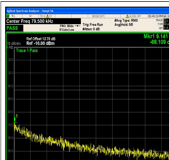
1-N25-PC3-15-15-L-21-CP-16QAM-Outer_F ull-79@0-0.009-0.15-Ant1--68.11--43-PASS
