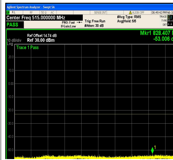
1-N25-PC3-15-15-L-21-CP-16QAM-Outer_F ull-79@0-30-1000-Ant1--53.01--23-PASS
