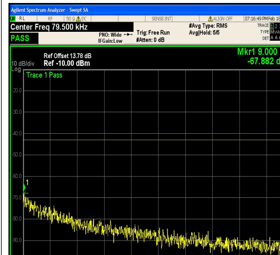
1-N25-PC3-15-15-M-8-DFT-16QAM-Edge_1 RB_Right-1@78-0.009-0.15-Ant1--67.88--43-P PASS
