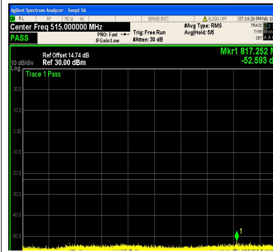
1-N25-PC3-15-15-M-6-DFT-QPSK-Outer_Ful I-75@0-30-1000-Ant1--52.59--23-PASS
