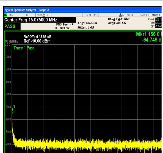
1-N25-PC3-15-15-M-6-DFT-QPSK-Outer_Ful I-75@0-0.15-30-Ant1--64.75--33-PASS
