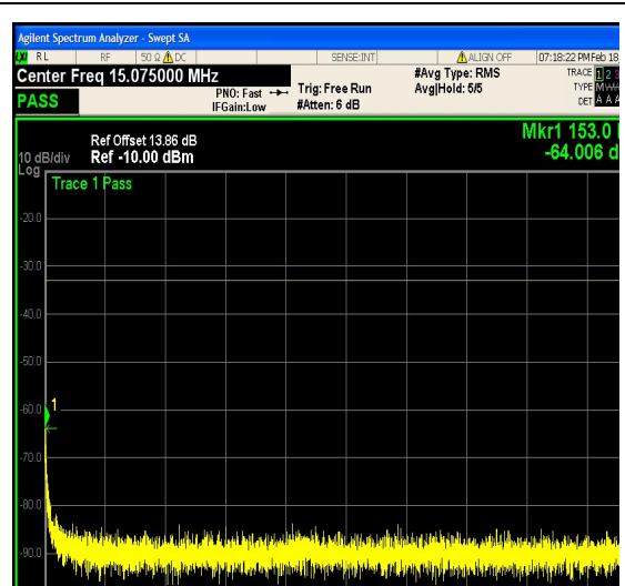
1-N25-PC3-15-15-M-9-DFT-16QAM-Outer_F ull-75@0-0.15-30-Ant1--64.01--33-PASS
