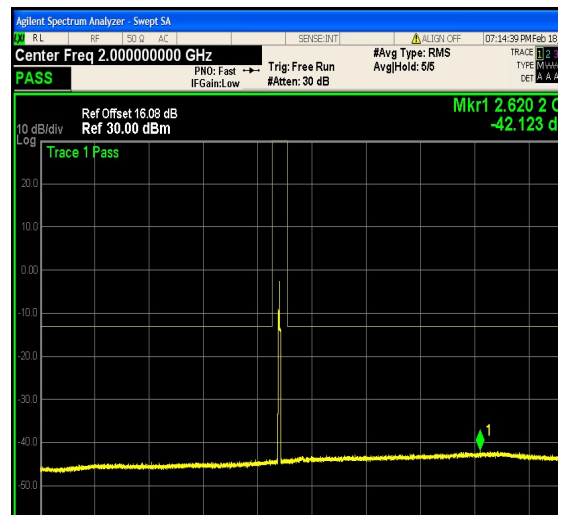
1-N25-PC3-15-15-M-6-DFT-QPSK-Outer_Ful I-75@0-1000-3000-Ant1--42.12--13-PASS
