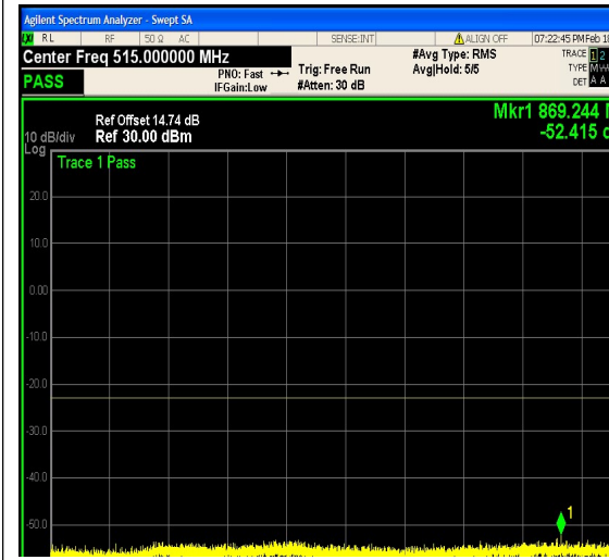
1-N25-PC3-15-15-M-12-DFT-64QAM-Outer_ Full-75@0-30-1000-Ant1--52.41--23-PASS
