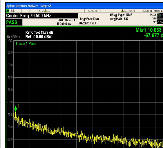
1-N25-PC3-15-15-M-18-CP-QPSK-Outer_Ful l-79@0-0.009-0.15-Ant1--67.98--43-PASS
