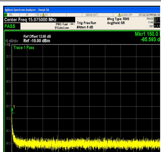
1-N25-PC3-15-15-M-12-DFT-64QAM-Outer_ Full-75@0-0.15-30-Ant1--65.59--33-PASS
