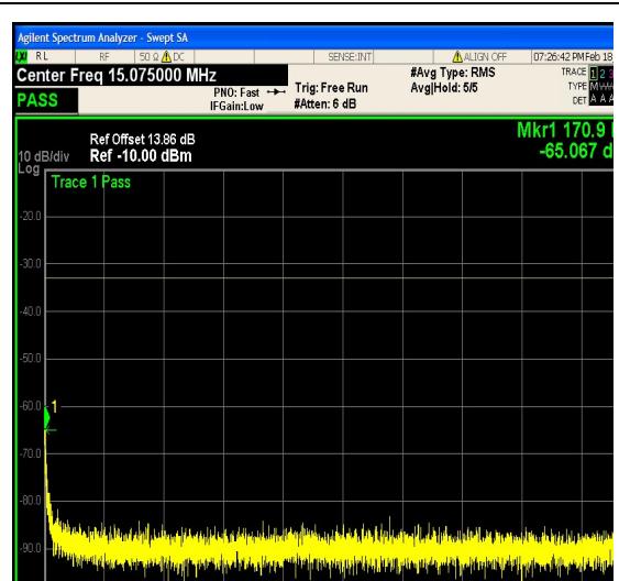
1-N25-PC3-15-15-M-15-DFT-256QAM-Outer _Full-75@0-0.15-30-Ant1--65.07--33-PASS
