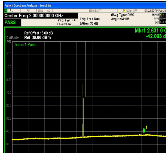
1-N25-PC3-15-15-M-12-DFT-64QAM-Outer_ Full-75@0-1000-3000-Ant1--42.09--13-PASS
