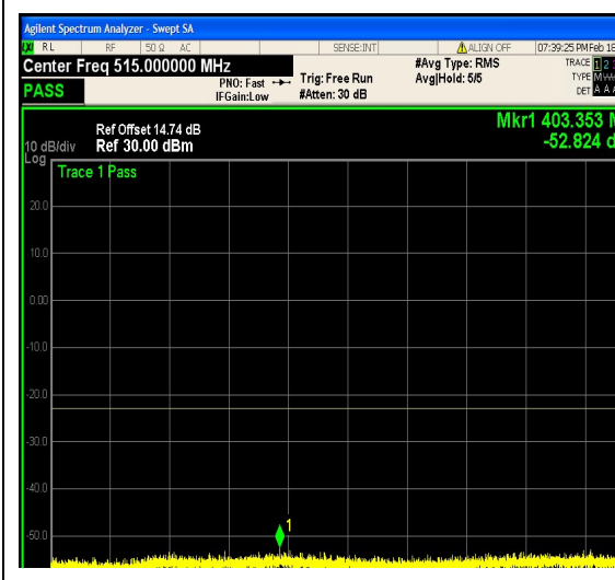
1-N25-PC3-15-15-M-24-CP-64QAM-Outer_F ull-79@0-0.009-0.15-Ant1--68.09--43-PASS
