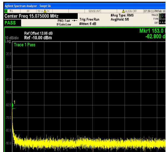
1-N25-PC3-15-15-M-24-CP-64QAM-Outer_F ull-79@0-0.15-30-Ant1--62.80--33-PASS
