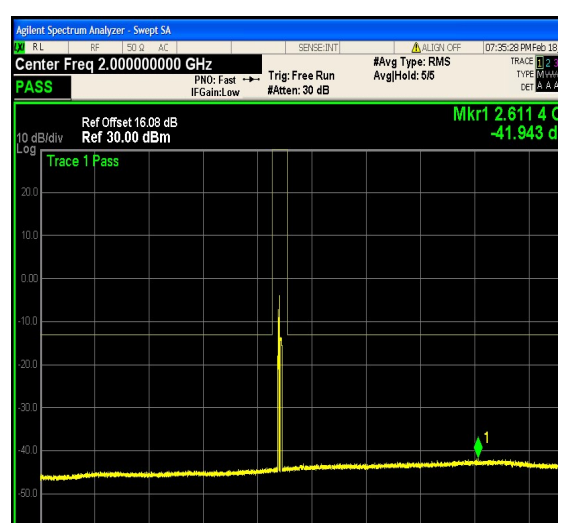
1-N25-PC3-15-15-M-21-CP-16QAM-Outer_F ull-79@0-0.15-30-Ant1--64.88--33-PASS
