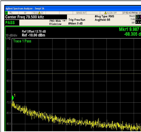
1-N25-PC3-15-15-H-5-DFT-QPSK-Edge_1R B_Right-1@78-0.009-0.15-Ant1--68.30--43-P ASS
