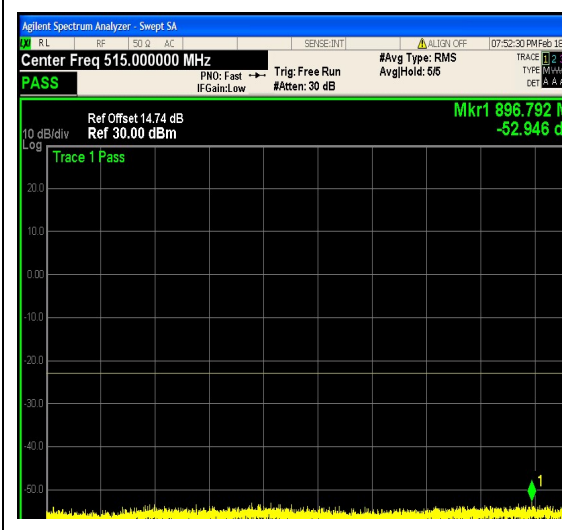
1-N25-PC3-15-15-H-6-DFT-QPSK-Outer_Full -75@0-0.009-0.15-Ant1--68.54--43-PASS
