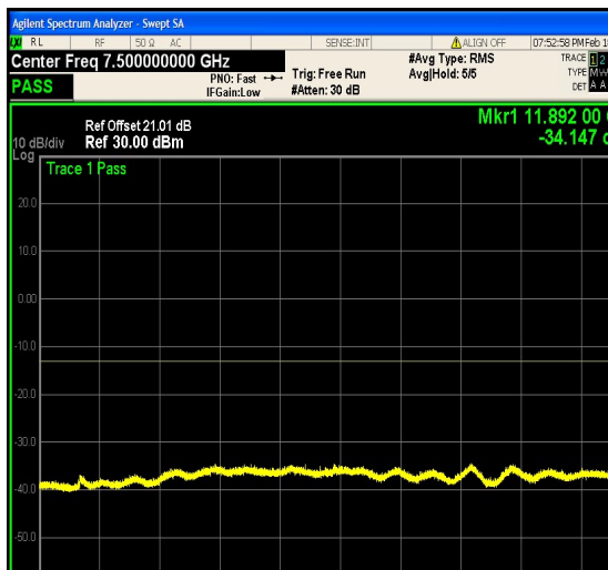
1-N25-PC3-15-15-H-6-DFT-QPSK-Outer_Full -75@0-3000-12000-Ant1--34.15--13-PASS
