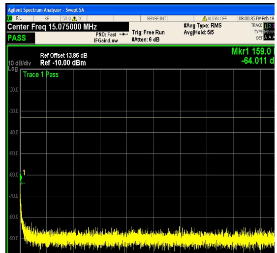
1-N25-PC3-15-15-H-12-DFT-64QAM-Outer_ Full-75@0-0.15-30-Ant1--64.01--33-PASS
