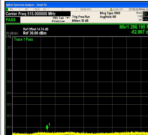
1-N25-PC3-15-15-H-11-DFT-64QAM-Edge_1 RB_Right-1@78-30-1000-Ant1--52.87--23-P ASS
