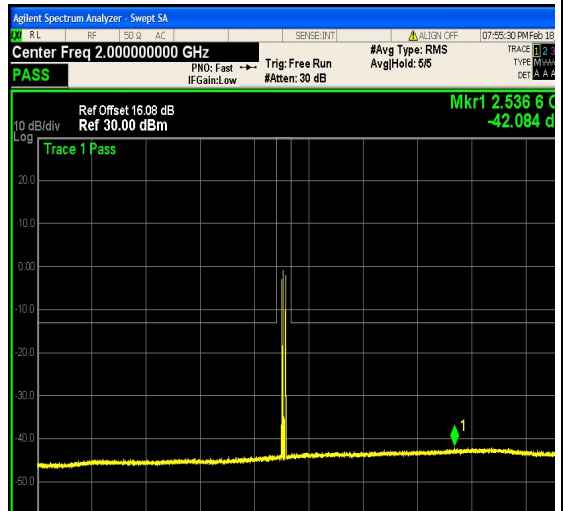
1-N25-PC3-15-15-H-8-DFT-16QAM-Edge_1 RB_Right-1@78-1000-3000-Ant1--42.08--13- PASS
