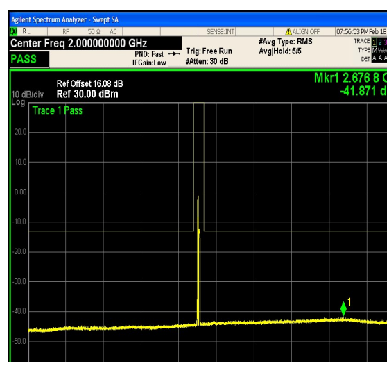
1-N25-PC3-15-15-H-9-DFT-16QAM-Outer_F ull-75@0-0.15-30-Ant1--63.38--33-PASS
