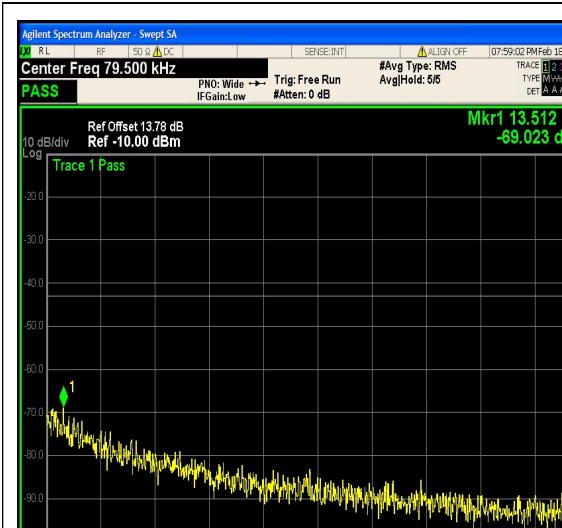
1-N25-PC3-15-15-H-11-DFT-64QAM-Edge_1 RB_Right-1@78-0.009-0.15-Ant1--69.02--43- PASS
