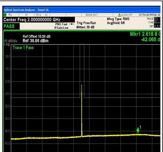
1-N25-PC3-15-15-H-7-DFT-16QAM-Edge_1 RB_Left-1@0-1000-3000-Ant1--42.06--13-PA SS
