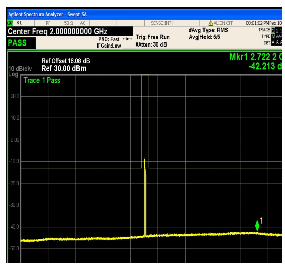
1-N25-PC3-15-15-H-12-DFT-64QAM-Outer_ Full-75@0-0.15-30-Ant1--64.01--33-PASS
