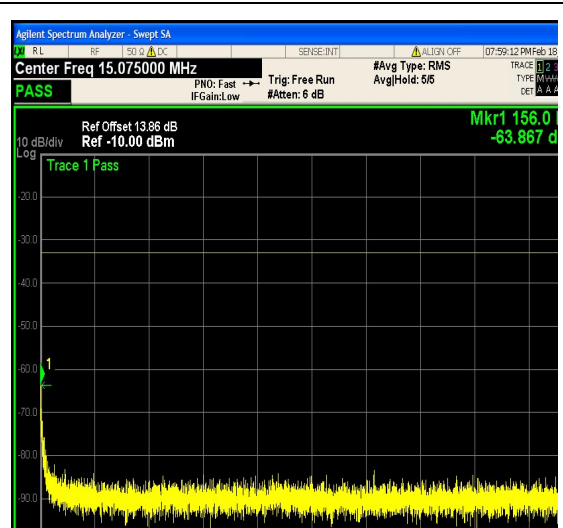
1-N25-PC3-15-15-H-11-DFT-64QAM-Edge_1 RB_Right-1@78-0.15-30-Ant1--63.87--33-PA SS
