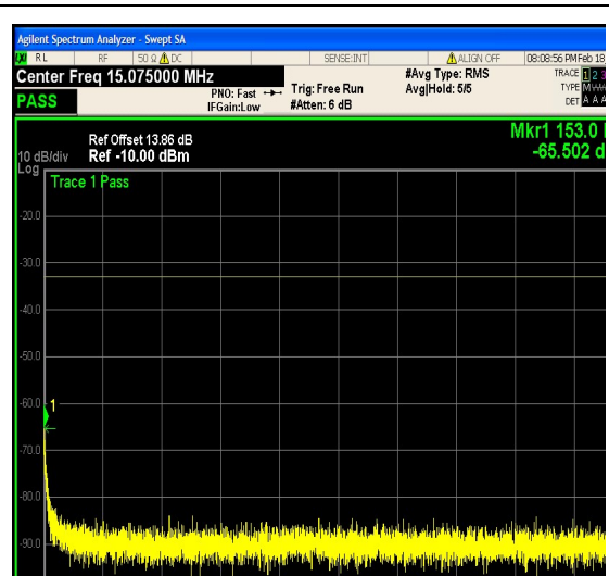
1-N25-PC3-15-15-H-18-CP-QPSK-Outer_Ful I-79@0-0.15-30-Ant1--65.50--33-PASS
