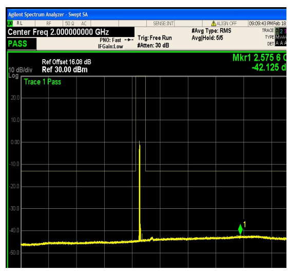
1-N25-PC3-15-20-L-24-CP-64QAM-Outer_F ull-106@0-0.15-30-Ant1--64.90--33-PASS
