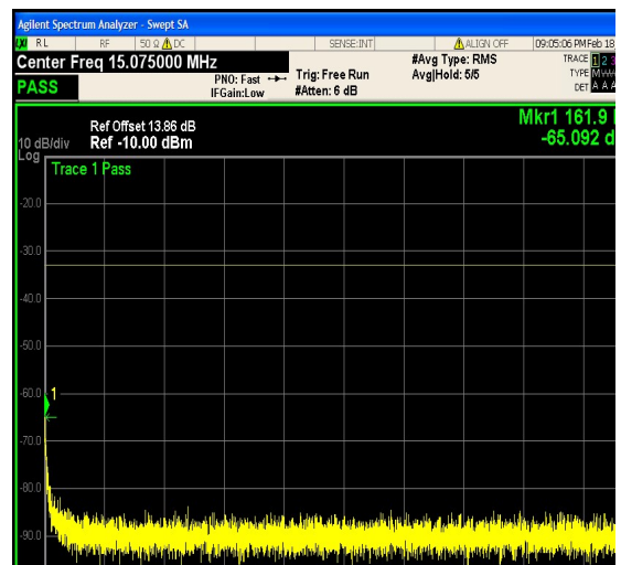
1-N25-PC3-15-20-L-21-CP-16QAM-Outer_F ull-106@0-0.15-30-Ant1--65.09--33-PASS
