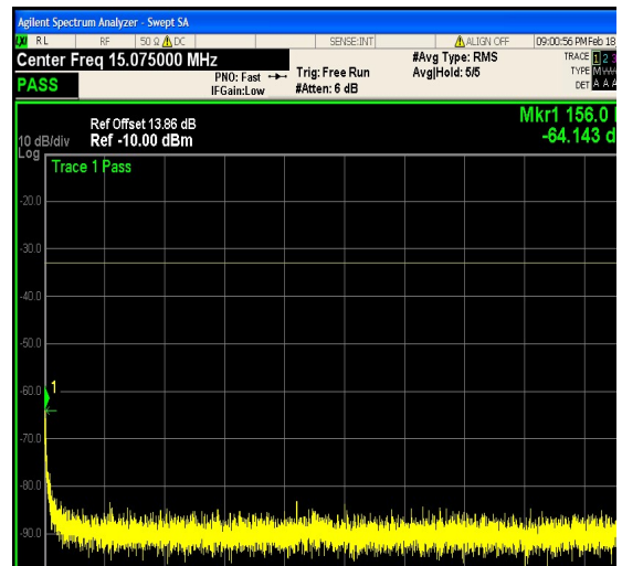
1-N25-PC3-15-20-L-18-CP-QPSK-Outer_Full -106@0-0.15-30-Ant1--64.14--33-PASS
