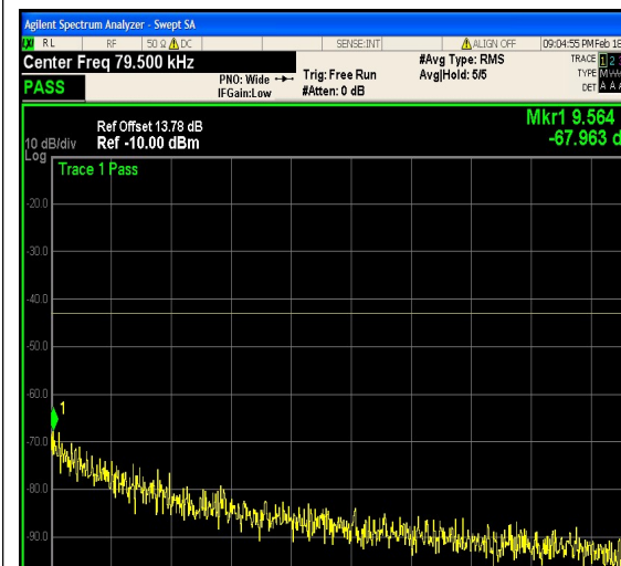
1-N25-PC3-15-20-L-21-CP-16QAM-Outer_F ull-106@0-0.009-0.15-Ant1--67.96--43-PASS
