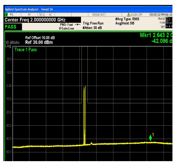
1-N25-PC3-15-20-L-21-CP-16QAM-Outer_F ull-106@0-0.15-30-Ant1--65.09--33-PASS
