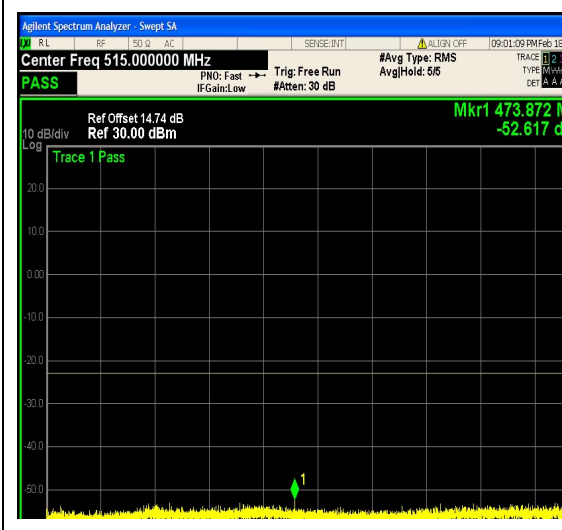
1-N25-PC3-15-20-L-18-CP-QPSK-Outer_Full -106@0-0.009-0.15-Ant1--69.41--43-PASS
