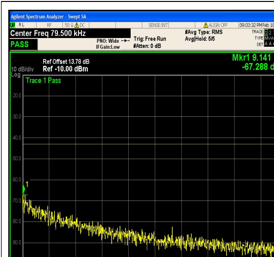
1-N25-PC3-15-20-L-20-CP-16QAM-Edge_1R B_Right-1@105-0.009-0.15-Ant1--67.29--43- PASS
