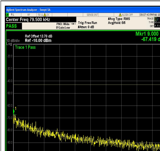
1-N25-PC3-15-20-L-23-CP-64QAM-Edge_1R B_Right-1@105-0.009-0.15-Ant1--67.42--43- PASS
