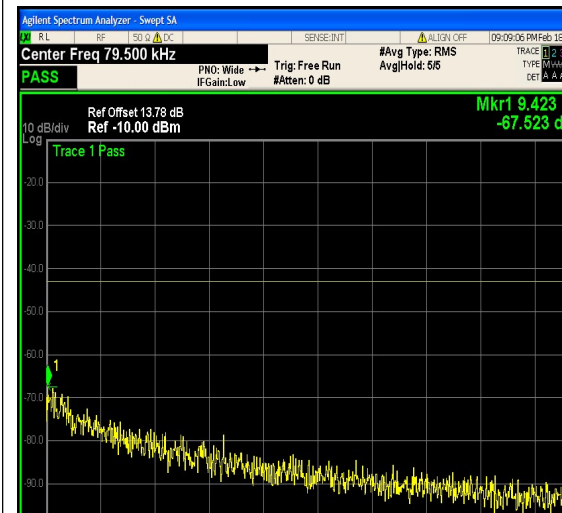
1-N25-PC3-15-20-L-24-CP-64QAM-Outer_F ull-106@0-0.009-0.15-Ant1--67.52--43-PASS
