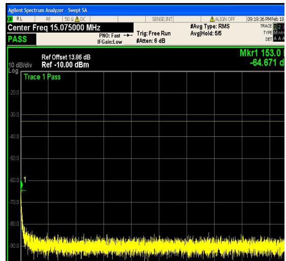
1-N25-PC3-15-20-M-4-DFT-QPSK-Edge_1R B_Left-1@0-0.15-30-Ant1--64.67--33-PASS
