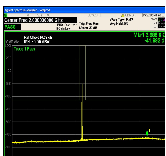
1-N25-PC3-15-20-M-4-DFT-QPSK-Edge_1R B_Left-1@0-1000-3000-Ant1--41.89--13-PASS
