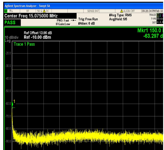
1-N25-PC3-15-20-M-9-DFT-16QAM-Outer_F ull-100@0-0.15-30-Ant1--63.30--33-PASS
