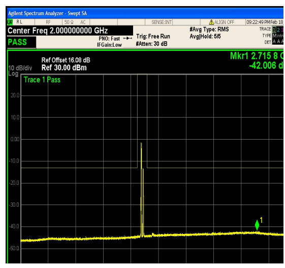
1-N25-PC3-15-20-M-6-DFT-QPSK-Outer_Ful l-100@0-0.15-30-Ant1--65.76--33-PASS
