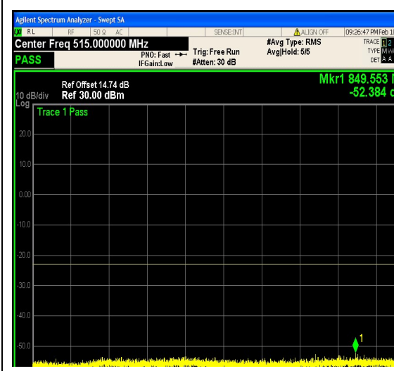
1-N25-PC3-15-20-M-9-DFT-16QAM-Outer_F ull-100@0-0.009-0.15-Ant1--61.92--43-PASS
