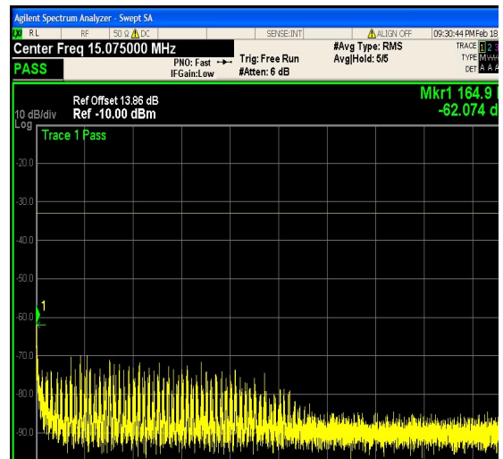
1-N25-PC3-15-20-M-12-DFT-64QAM-Outer_ Full-100@0-0.15-30-Ant1--62.07--33-PASS
